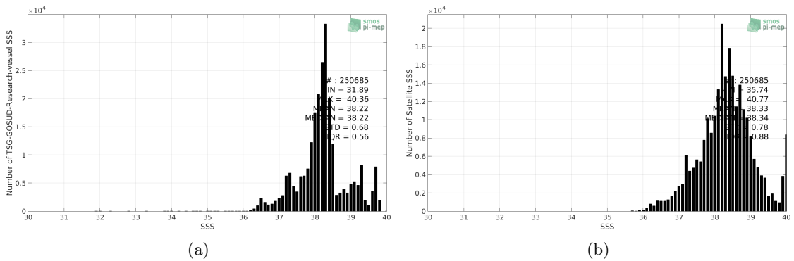
Figure 2: Histograms of SSS from TSG-GOSUD-Research-vessel (a) and CCI L4 Merged-OI v1.8 - 7-day running (ESA) (b) considering all match-up pairs per bins of 0.1 over the Mediterranean Sea Pi-MEP region and for the full satellite product period.
