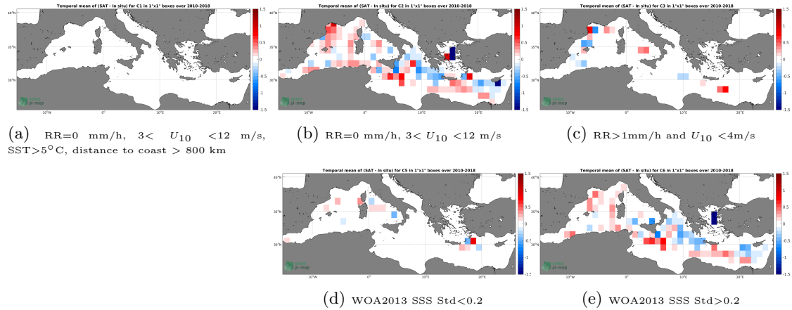
Figure 12: Temporal mean gridded over spatial boxes of size 1^{\circ}\times 1^{\circ} of \Delta SSS (CCI L4 Merged-OI v1.8 - 7-day running (ESA) - TSG-GOSUD-Research-vessel) for 5 different subdatasets corresponding to:RR=0 mm/h, 3 < U_{10} < 12 m/s, SST >5^{\circ}\text{C} , distance to coast > 800 km (a), RR=0 mm/h, 3 < U_{10} < 12 m/s (b), RR >1 mm/h and U_{10} < 4 m/s (c), WOA2013 SSS Std <0.2 (d), WOA2013 SSS Std >0.2 (e).
