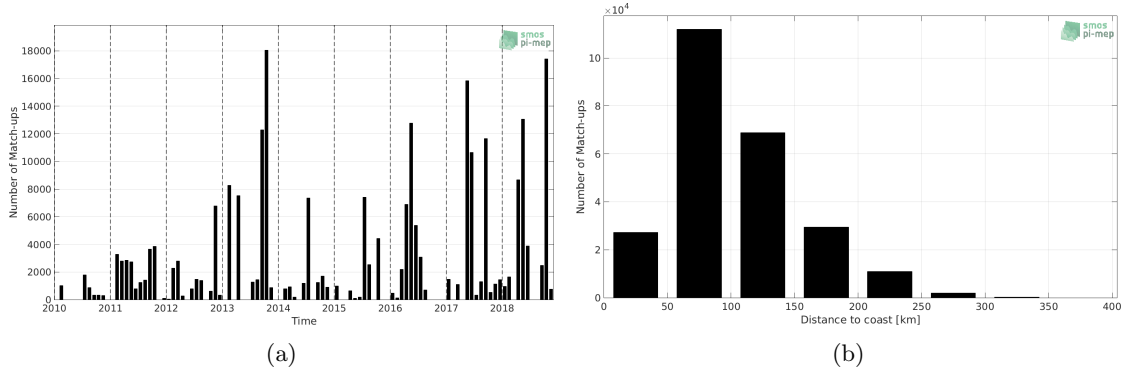
Figure 1: Number of match-ups between TSG-GOSUD-Research-vessel and CCI L4 Merged-OI v1.8 - 7-day running (ESA) SSS as a function of time (a) and as function of the distance to coast (b) over the Mediterranean Sea Pi-MEP region and for the full satellite product period.
