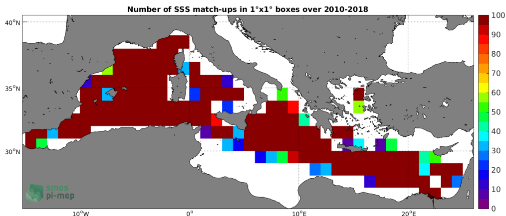
Figure 4: Number of SSS match-ups between TSG-GOSUD-Research-vessel SSS and the CCI L4 Merged-OI v1.8 - 7-day running (ESA) SSS product for the Mediterranean Sea Pi-MEP region over 1^\circ \times 1^\circ boxes and for the full satellite product period.
