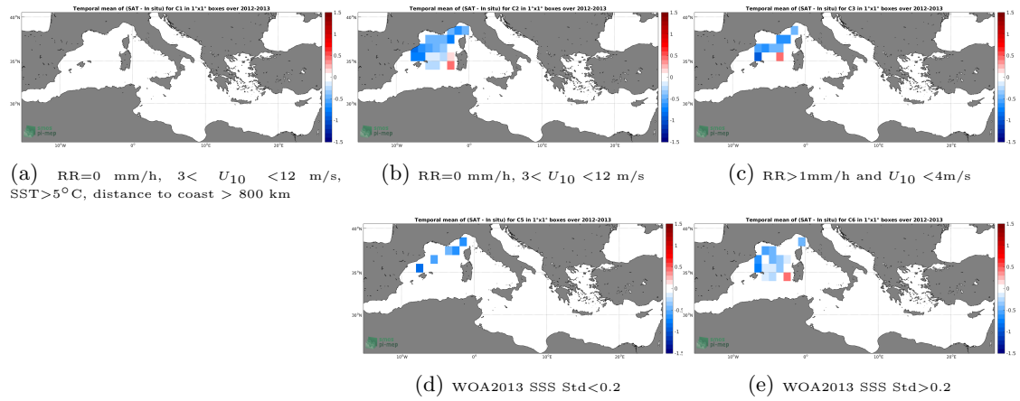
Figure 11: Temporal mean gridded over spatial boxes of size 1^\circ \times 1^\circ of \Delta SSS (CCI-L4-ESAMERGED-OI-V1.8-7DAY-RUNNING - Surface drifters) for 5 different subdatasets corresponding to:RR=0 mm/h, 3 < U_{10} < 12 m/s, SST >5^\circ\text{C} , distance to coast > 800 km (a), RR=0 mm/h, 3 < U_{10} < 12 m/s (b), RR >1 mm/h and U_{10} < 4 m/s (c), WOA2013 SSS Std <0.2 (d), WOA2013 SSS Std >0.2 (e).
