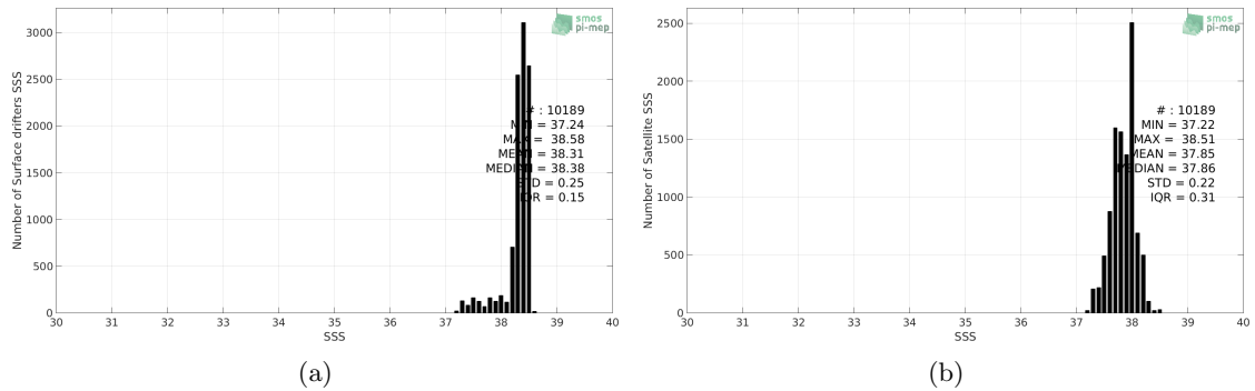
Figure 2: Histograms of SSS from Surface drifters (a) and CCI-L4-ESA-MERGED-OI-V1.8-7DAY-RUNNING (b) considering all match-up pairs per bins of 0.1 over the Mediterranean Sea Pi-MEP region and for the full satellite product period.
