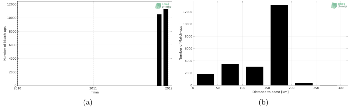
Figure 1: Number of match-ups between TSG-SAMOS and CCI-L4-ESA-MERGED-OI-V1.8-30DAY-RUNNING SSS as a function of time (a) and as function of the distance to coast (b) over the Mediterranean Sea Pi-MEP region and for the full satellite product period.
