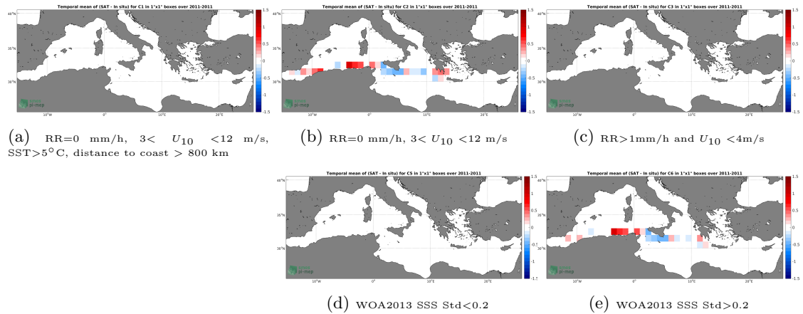
Figure 12: Temporal mean gridded over spatial boxes of size 1^\circ \times 1^\circ of \Delta SSS (CCI-L4-ESAMERGED-OI-V1.8-30DAY-RUNNING - TSG-SAMOS) for 5 different subdatasets corresponding to:RR=0 mm/h, 3 < U_{10} < 12 m/s, SST >5^\circ\text{C} , distance to coast > 800 km (a), RR=0 mm/h, 3 < U_{10} < 12 m/s (b), RR >1 mm/h and U_{10} < 4 m/s (c), WOA2013 SSS Std <0.2 (d), WOA2013 SSS Std >0.2 (e).
