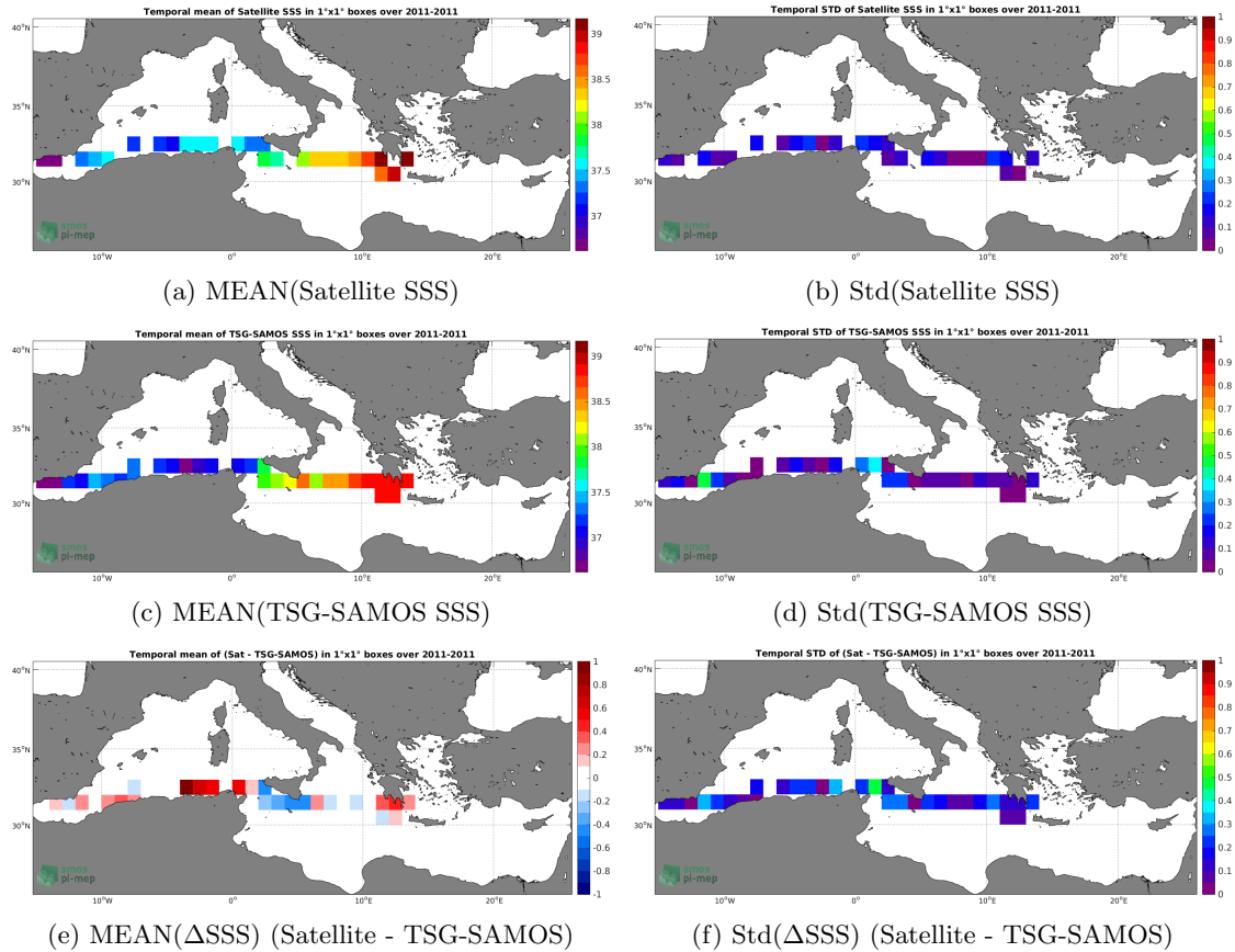
Figure 6: Temporal mean (left) and Std (right) of SSS from CCI-L4-ESA-MERGED-OI-V1.8-30DAY-RUNNING (top), TSG-SAMOS (middle), and of \Delta SSS (Satellite - TSG-SAMOS). Only match-up pairs are used to generate these maps.
