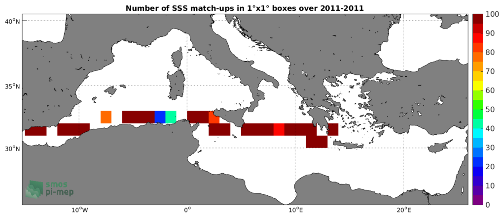
Figure 4: Number of SSS match-ups between TSG-SAMOS SSS and the CCI-L4-ESA-MERGED-OI-V1.8-30DAY-RUNNING SSS product for the Mediterranean Sea Pi-MEP region over 1^\circ \times 1^\circ boxes and for the full satellite product period.
