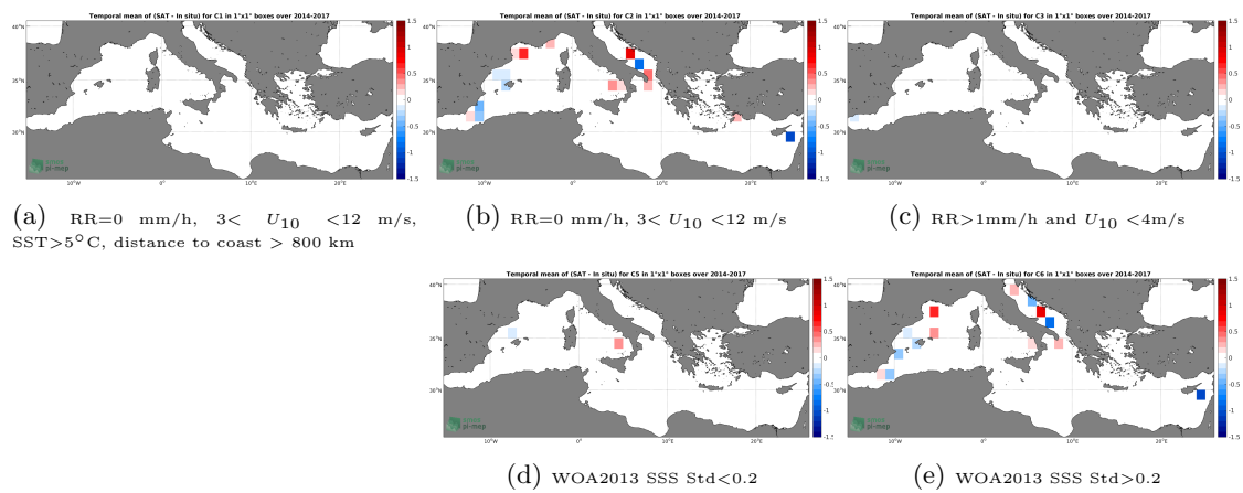
Figure 12: Temporal mean gridded over spatial boxes of size 1^\circ \times 1^\circ of \Delta SSS (CCI-L4-ESA-MERGED-OI-V1.8-30DAY-RUNNING - TSG-GOSUD-Sailing-ship) for 5 different subdatasets corresponding to:RR=0 mm/h, 3 < U_{10} < 12 m/s, SST >5^\circ\text{C} , distance to coast > 800 km (a), RR=0 mm/h, 3 < U_{10} < 12 m/s (b), RR >1 mm/h and U_{10} < 4 m/s (c), WOA2013 SSS Std <0.2 (d), WOA2013 SSS Std >0.2 (e).
