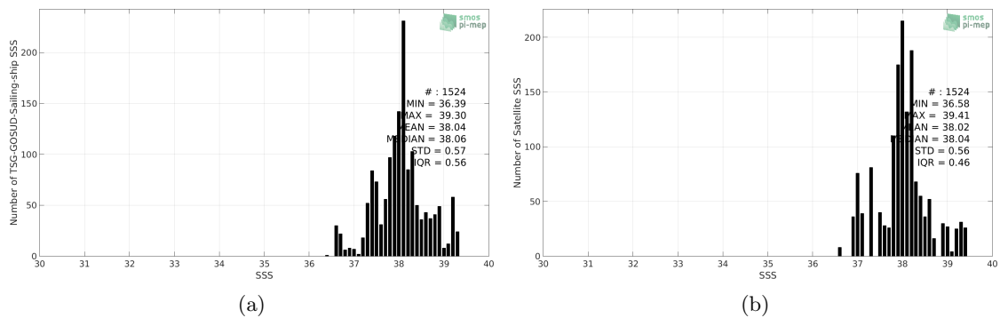
Figure 2: Histograms of SSS from TSG-GOSUD-Sailing-ship (a) and CCI-L4-ESA-MERGED-OI-V1.8-30DAY-RUNNING (b) considering all match-up pairs per bins of 0.1 over the Mediterranean Sea Pi-MEP region and for the full satellite product period.
