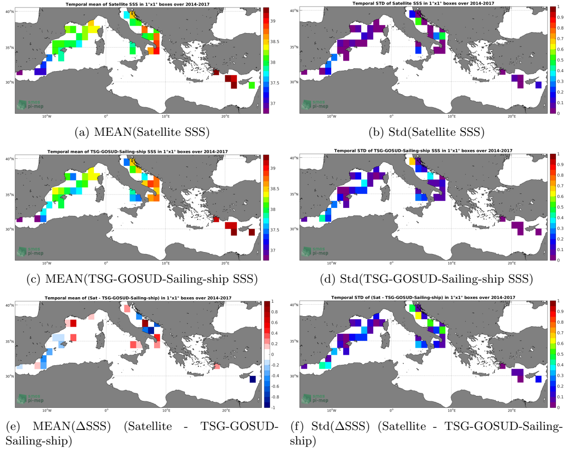
Figure 6: Temporal mean (left) and Std (right) of SSS from CCI-L4-ESA-MERGED-OI-V1.8-30DAY-RUNNING (top), TSG-GOSUD-Sailing-ship (middle), and of \Delta SSS (Satellite - TSG-GOSUD-Sailing-ship). Only match-up pairs are used to generate these maps.
