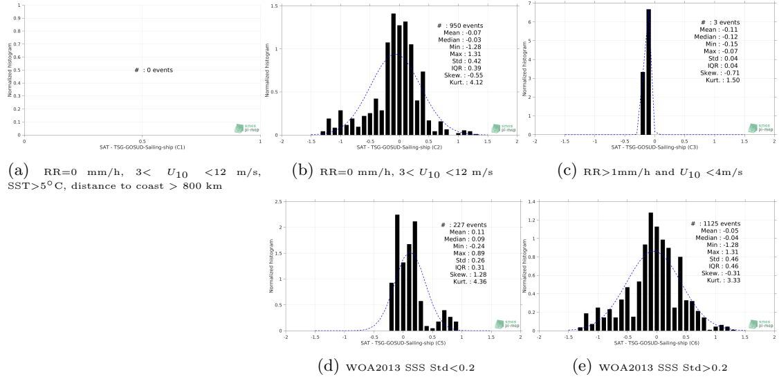
Figure 13: Normalized histogram of \Delta SSS (CCI-L4-ESA-MERGED-OI-V1.8-30DAY-RUNNING - TSG-GOSUD-Sailing-ship) for 5 different subdatasets corresponding to: RR=0 mm/h, 3 < U_{10} < 12 m/s, SST>5°C, distance to coast > 800 km (a), RR=0 mm/h, 3 < U_{10} < 12 m/s (b), RR>1mm/h and U_{10} < 4 m/s (c), WOA2013 SSS Std<0.2 (d), WOA2013 SSS Std>0.2 (e).
