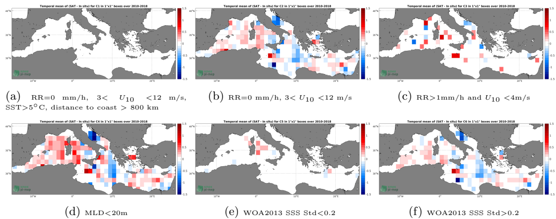
Figure 12: Temporal mean gridded over spatial boxes of size 1^\circ \times 1^\circ of \Delta SSS (CCI-L4-ESA-MERGED-OI-V1.8-30DAY-RUNNING - Argo) for 6 different subdatasets corresponding to:RR=0 mm/h, 3 < U_{10} < 12 m/s, SST >5^\circ C, distance to coast > 800 km (a), RR=0 mm/h, 3 < U_{10} < 12 m/s (b), RR >1 mm/h and U_{10} < 4 m/s (c),MLD <20 m (d),WOA2013 SSS Std <0.2 (e),WOA2013 SSS Std >0.2 (f).
