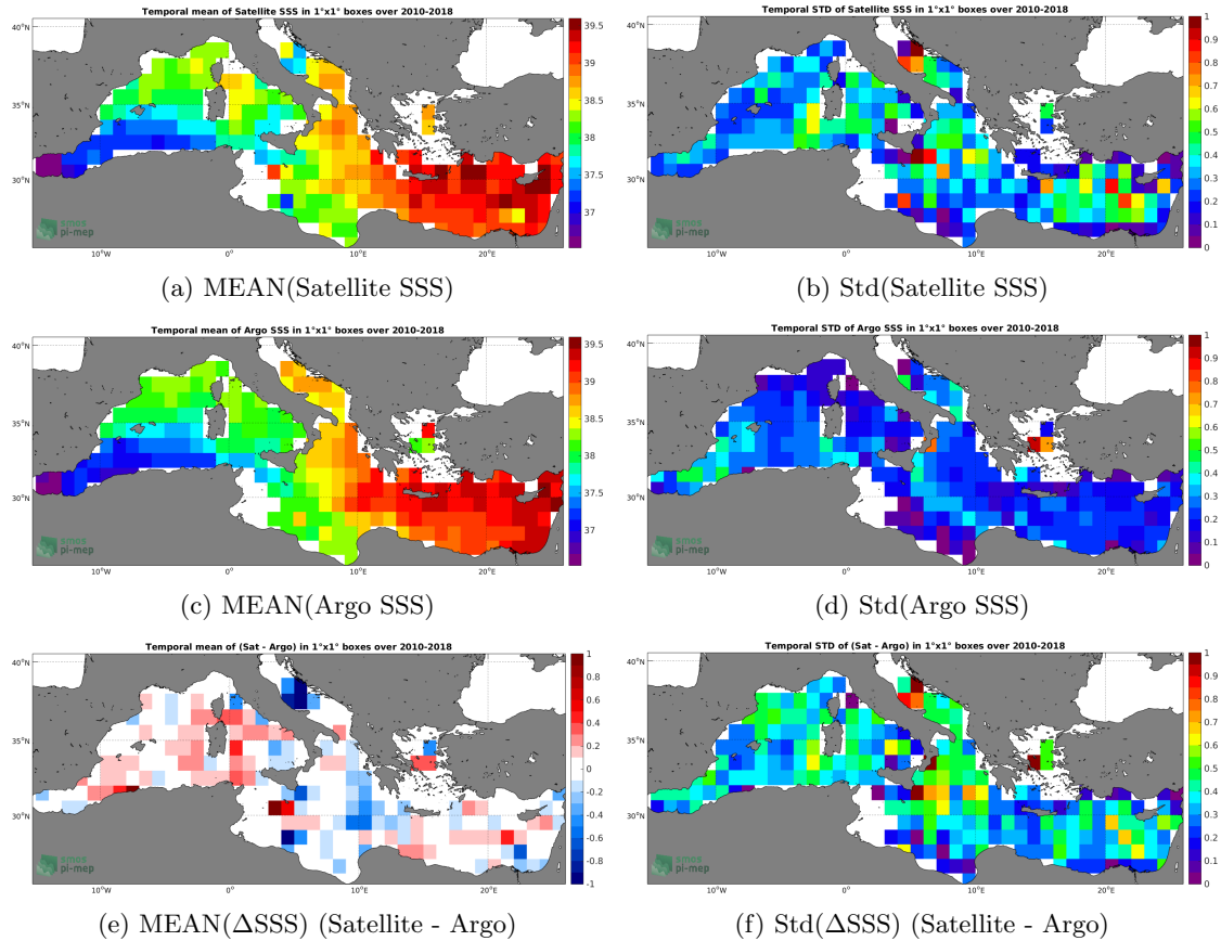
Figure 6: Temporal mean (left) and Std (right) of SSS from CCI-L4-ESA-MERGED-OI-V1.8-30DAY-RUNNING (top), Argo (middle), and of \Delta SSS (Satellite - Argo). Only match-up pairs are used to generate these maps.
