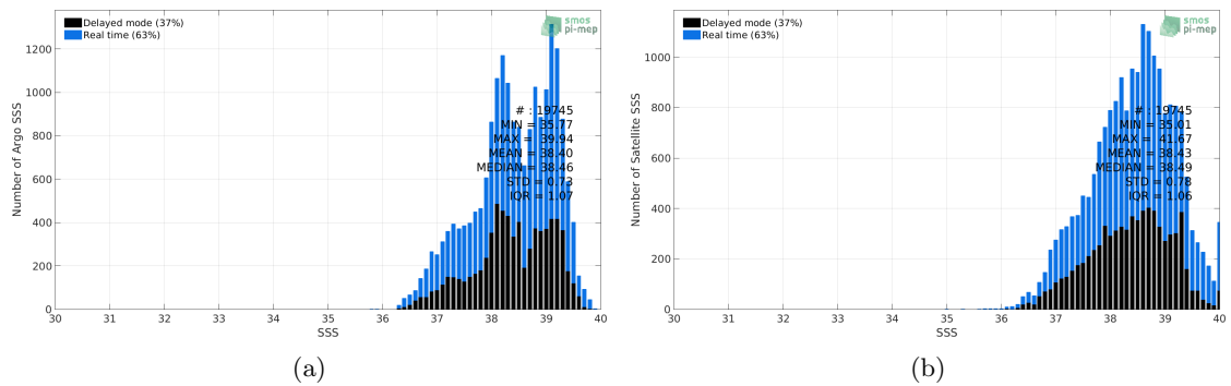
Figure 2: Histograms of SSS from Argo (a) and CCI-L4-ESA-MERGED-OI-V1.8-30DAY-RUNNING (b) considering all match-up pairs per bins of 0.1 over the Mediterranean Sea Pi-MEP region and for the full satellite product period.
