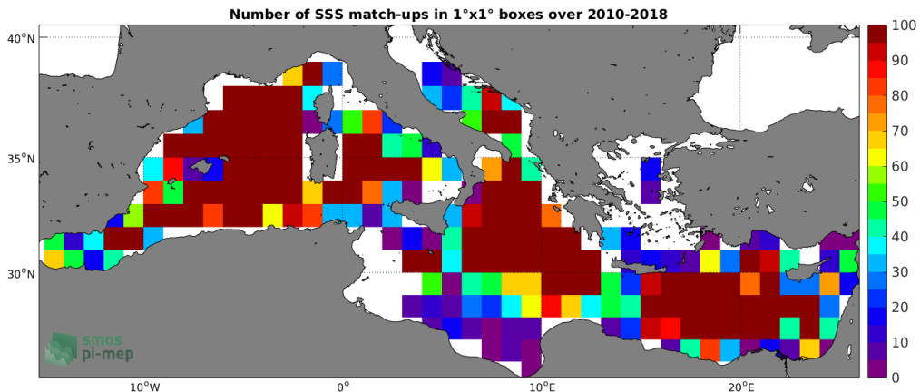
Figure 4: Number of SSS match-ups between Argo SSS and the CCI-L4-ESA-MERGED-OI-V1.8-30DAY-RUNNING SSS product for the Mediterranean Sea Pi-MEP region over 1°x1° boxes and for the full satellite product period.
