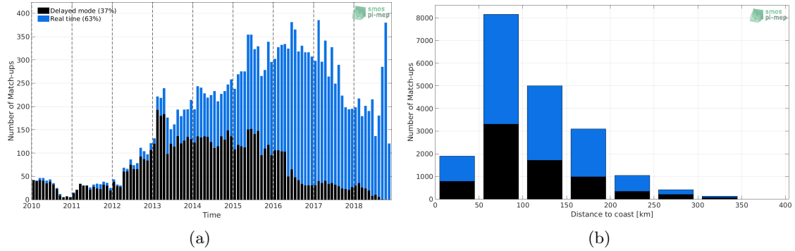
Figure 1: Number of match-ups between Argo and CCI-L4-ESA-MERGED-OI-V1.8-30DAY-RUNNING SSS as a function of time (a) and as function of the distance to coast (b) over the Mediterranean Sea Pi-MEP region and for the full satellite product period.
