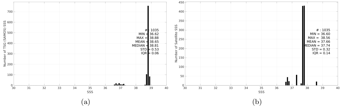
Figure 3: Histograms of SSS from TSG (SAMOS) (a) and Aquarius SSS L3 OR v5 - 7-Day running (NASA-GSFC) (b) considering all match-up pairs per bins of 0.1 over the Mediterranean Sea Pi-MEP region and for the full satellite product period.
