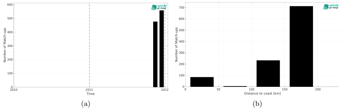
Figure 2: Number of match-ups between TSG (SAMOS) and Aquarius SSS L3 OR v5 - 7-Day running (NASA-GSFC) SSS as a function of time (a) and as function of the distance to coast (b) over the Mediterranean Sea Pi-MEP region and for the full satellite product period.
