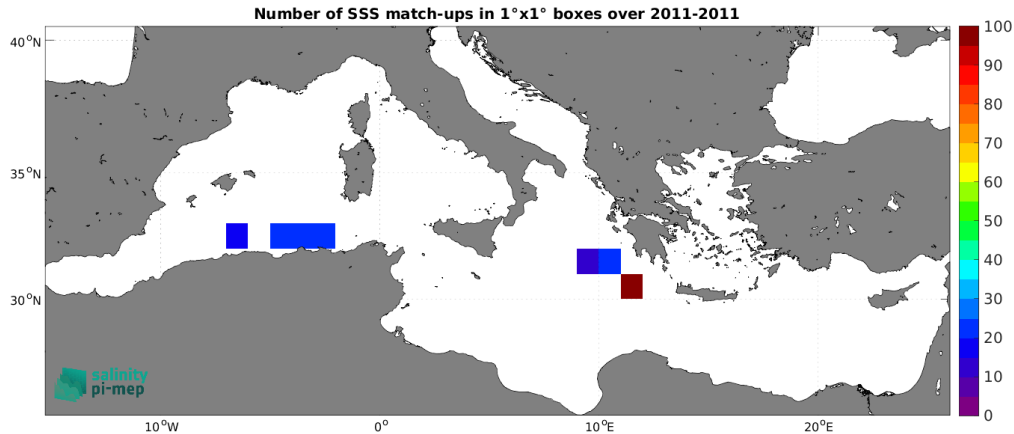
Figure 5: Number of SSS match-ups between TSG (SAMOS) SSS and the Aquarius SSS L3 OR v5 - 7-Day running (NASA-GSFC) SSS product for the Mediterranean Sea Pi-MEP region over 1^\circ \times 1^\circ boxes and for the full satellite product period.
