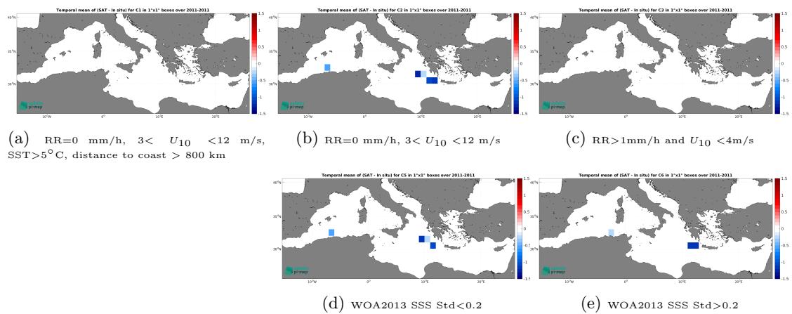
Figure 14: Temporal mean gridded over spatial boxes of size 1^\circ \times 1^\circ of \Delta\text{SSS} (Aquarius SSS L3 OR v5 - 7-Day running (NASA-GSFC) - TSG (SAMOS)) for 5 different subdatasets corresponding to:RR=0 mm/h, 3 < U_{10} < 12 m/s, SST>5°C, distance to coast > 800 km (a), RR=0 mm/h, 3 < U_{10} < 12 m/s (b), RR>1mm/h and U_{10} < 4 m/s (c), WOA2013 SSS Std<0.2 (d), WOA2013 SSS Std>0.2 (e).
