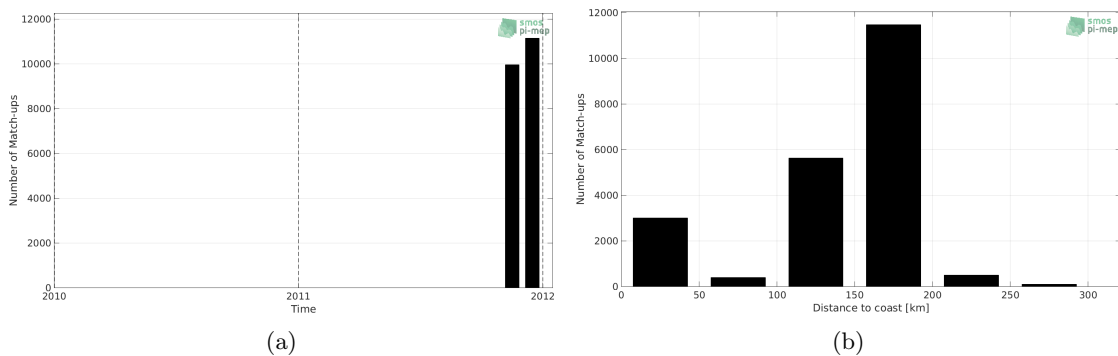
Figure 1: Number of match-ups between TSG-SAMOS and Aquarius-L3-OR-V5-7DAY-RUNNING-1DEG SSS as a function of time (a) and as function of the distance to coast (b) over the Mediterranean Sea Pi-MEP region and for the full satellite product period.
