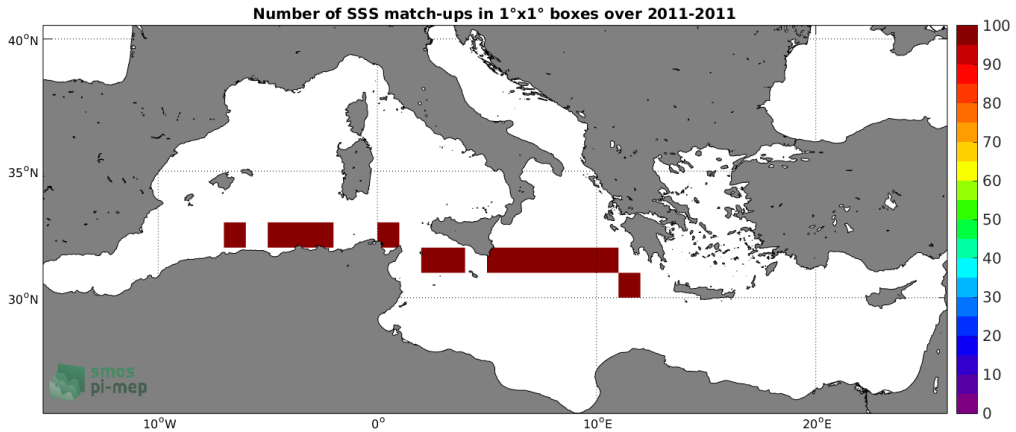
Figure 4: Number of SSS match-ups between TSG-SAMOS SSS and the Aquarius-L3-OR-V5-7DAY-RUNNING-1DEG SSS product for the Mediterranean Sea Pi-MEP region over 1^\circ \times 1^\circ boxes and for the full satellite product period.
