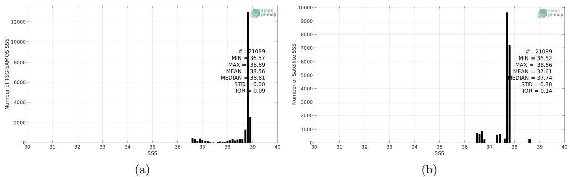
Figure 2: Histograms of SSS from TSG-SAMOS (a) and Aquarius-L3-OR-V5-7DAY-RUNNING-1DEG (b) considering all match-up pairs per bins of 0.1 over the Mediterranean Sea Pi-MEP region and for the full satellite product period.
