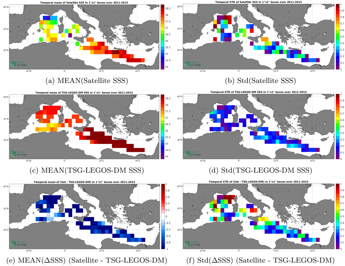
Figure 6: Temporal mean (left) and Std (right) of SSS from Aquarius-L3-OR-V5-7DAY-RUNNING-1DEG (top), TSG-LEGOS-DM (middle), and of \Delta SSS (Satellite - TSG-LEGOS-DM). Only match-up pairs are used to generate these maps.
