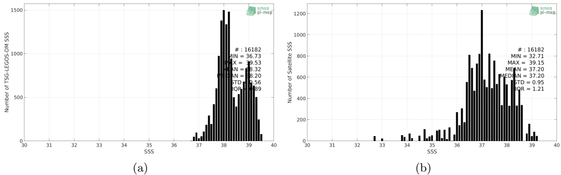
Figure 2: Histograms of SSS from TSG-LEGOS-DM (a) and Aquarius-L3-OR-V5-7DAY-RUNNING-1DEG (b) considering all match-up pairs per bins of 0.1 over the Mediterranean Sea Pi-MEP region and for the full satellite product period.
