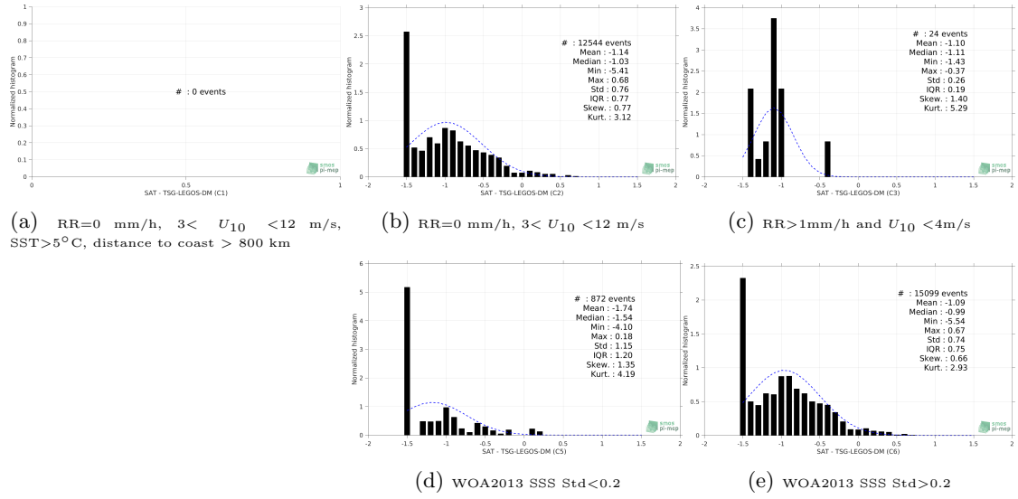
Figure 13: Normalized histogram of \Delta SSS (Aquarius-L3-OR-V5-7DAY-RUNNING-1DEG - TSG-LEGOS-DM) for 5 different subdatasets corresponding to: RR=0 mm/h, 3 < U_{10} < 12 m/s, SST > 5°C, distance to coast > 800 km (a), RR=0 mm/h, 3 < U_{10} < 12 m/s (b), RR > 1mm/h and U_{10} < 4 m/s (c), WOA2013 SSS Std < 0.2 (d), WOA2013 SSS Std > 0.2 (e).
