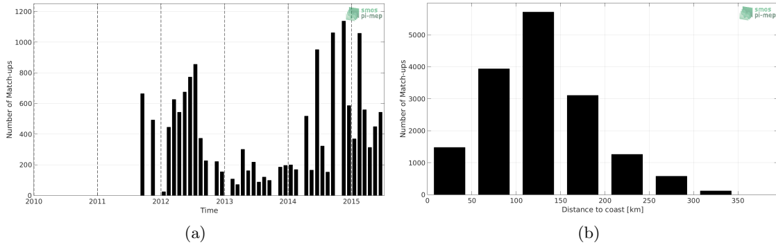
Figure 1: Number of match-ups between TSG-LEGOS-DM and Aquarius-L3-OR-V5-7DAY-RUNNING-1DEG SSS as a function of time (a) and as function of the distance to coast (b) over the Mediterranean Sea Pi-MEP region and for the full satellite product period.
