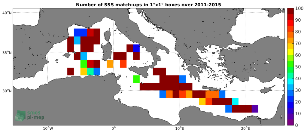
Figure 4: Number of SSS match-ups between TSG-LEGOS-DM SSS and the Aquarius-L3-OR-V5-7DAY-RUNNING-1DEG SSS product for the Mediterranean Sea Pi-MEP region over 1°x1° boxes and for the full satellite product period.
