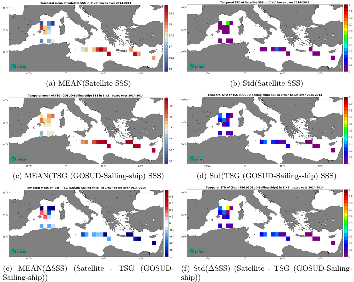
Figure 7: Temporal mean (left) and Std (right) of SSS from Aquarius SSS L3 OR v5 - 7-Day running (NASA-GSFC) (top), TSG (GOSUD-Sailing-ship) (middle), and of \Delta\text{SSS} (Satellite - TSG (GOSUD-Sailing-ship)). Only match-up pairs are used to generate these maps.
