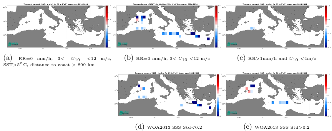
Figure 14: Temporal mean gridded over spatial boxes of size 1^\circ \times 1^\circ of \Delta SSS (Aquarius SSS L3 OR v5 - 7-Day running (NASA-GSFC) - TSG (GOSUD-Sailing-ship)) for 5 different subdatasets corresponding to:RR=0 mm/h, 3 < U_{10} < 12 m/s, SST>5°C, distance to coast > 800 km (a), RR=0 mm/h, 3 < U_{10} < 12 m/s (b), RR>1mm/h and U_{10} < 4 m/s (c), WOA2013 SSS Std<0.2 (d), WOA2013 SSS Std>0.2 (e).
