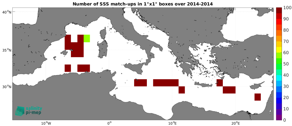
Figure 5: Number of SSS match-ups between TSG (GOSUD-Sailing-ship) SSS and the Aquarius SSS L3 OR v5 - 7-Day running (NASA-GSFC) SSS product for the Mediterranean Sea Pi-MEP region over 1^\circ \times 1^\circ boxes and for the full satellite product period.
