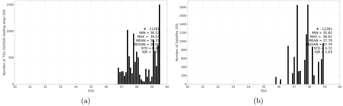
Figure 3: Histograms of SSS from TSG (GOSUD-Sailing-ship) (a) and Aquarius SSS L3 OR v5 - 7-Day running (NASA-GSFC) (b) considering all match-up pairs per bins of 0.1 over the Mediterranean Sea Pi-MEP region and for the full satellite product period.
