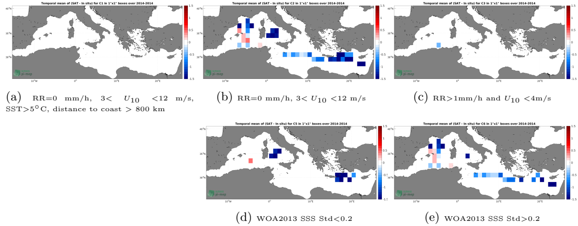
Figure 12: Temporal mean gridded over spatial boxes of size 1^{\circ}\times 1^{\circ} of \Delta SSS (Aquarius SSS L3 OR v5 - 7-Day running (NASA-GSFC) - TSG (GOSUD-Sailing-ship)) for 5 different subdatasets corresponding to: RR=0 mm/h, 3 < U_{10} < 12 m/s, SST > 5^{\circ}\text{C} , distance to coast > 800 km (a), RR=0 mm/h, 3 < U_{10} < 12 m/s (b), RR > 1 mm/h and U_{10} < 4 m/s (c), WOA2013 SSS Std < 0.2 (d), WOA2013 SSS Std > 0.2 (e).
