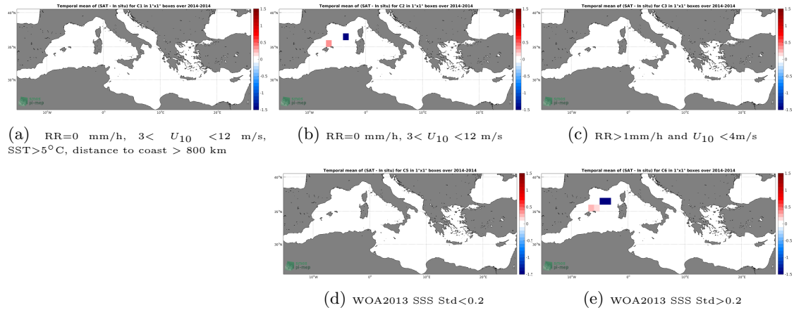
Figure 12: Temporal mean gridded over spatial boxes of size 1^{\circ}\times 1^{\circ} of \Delta SSS (Aquarius-L3-OR-V5-7DAY-RUNNING-1DEG - TSG-GOSUD-Sailing-ship) for 5 different subdatasets corresponding to:RR=0 mm/h, 3 < U_{10} < 12 m/s, SST >5^{\circ}\text{C} , distance to coast > 800 km (a), RR=0 mm/h, 3 < U_{10} < 12 m/s (b), RR >1 mm/h and U_{10} < 4 m/s (c), WOA2013 SSS Std <0.2 (d), WOA2013 SSS Std >0.2 (e).
