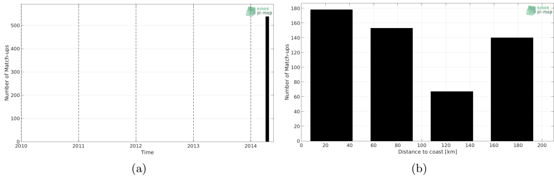
Figure 1: Number of match-ups between TSG-GOSUD-Sailing-ship and Aquarius-L3-OR-V5-7DAY-RUNNING-1DEG SSS as a function of time (a) and as function of the distance to coast (b) over the Mediterranean Sea Pi-MEP region and for the full satellite product period.
