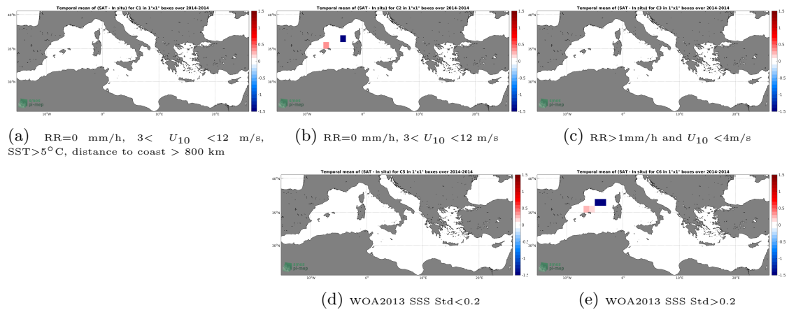
Figure 12: Temporal mean gridded over spatial boxes of size 1^\circ \times 1^\circ of \Delta SSS (Aquarius-L3-OR-V5-7DAY-RUNNING-1DEG - TSG-GOSUD-Sailing-ship) for 5 different subdatasets corresponding to:RR=0 mm/h, 3 < U_{10} < 12 m/s, SST >5^\circ\text{C} , distance to coast > 800 km (a), RR=0 mm/h, 3 < U_{10} < 12 m/s (b), RR >1 mm/h and U_{10} < 4 m/s (c), WOA2013 SSS Std <0.2 (d), WOA2013 SSS Std >0.2 (e).
