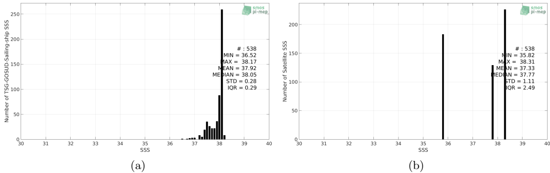
Figure 2: Histograms of SSS from TSG-GOSUD-Sailing-ship (a) and Aquarius-L3-OR-V5-7DAY-RUNNING-1DEG (b) considering all match-up pairs per bins of 0.1 over the Mediterranean Sea Pi-MEP region and for the full satellite product period.
