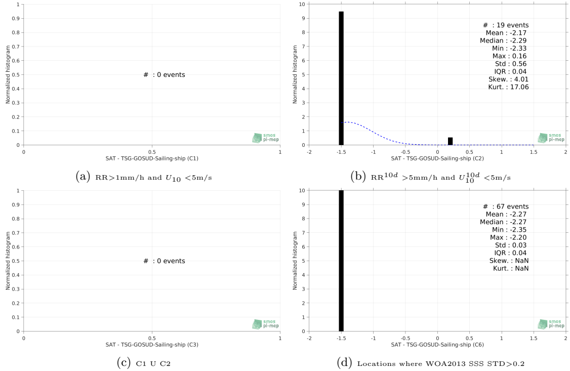
Figure 13: Normalized histogram of \Delta\text{SSS} (Aquarius-L3-OR-V5-7DAY-RUNNING-1DEG - TSG-GOSUD-Sailing-ship) for 6 different subdatasets corresponding to: RR > 1\text{mm/h} and U_{10} < 5\text{m/s} (a), RR^{10d} > 5\text{mm/h} and U_{10}^{10d} < 5\text{m/s} (b), C1 U C2 (c), Locations where WOA2013 SSS STD > 0.2 (d).
