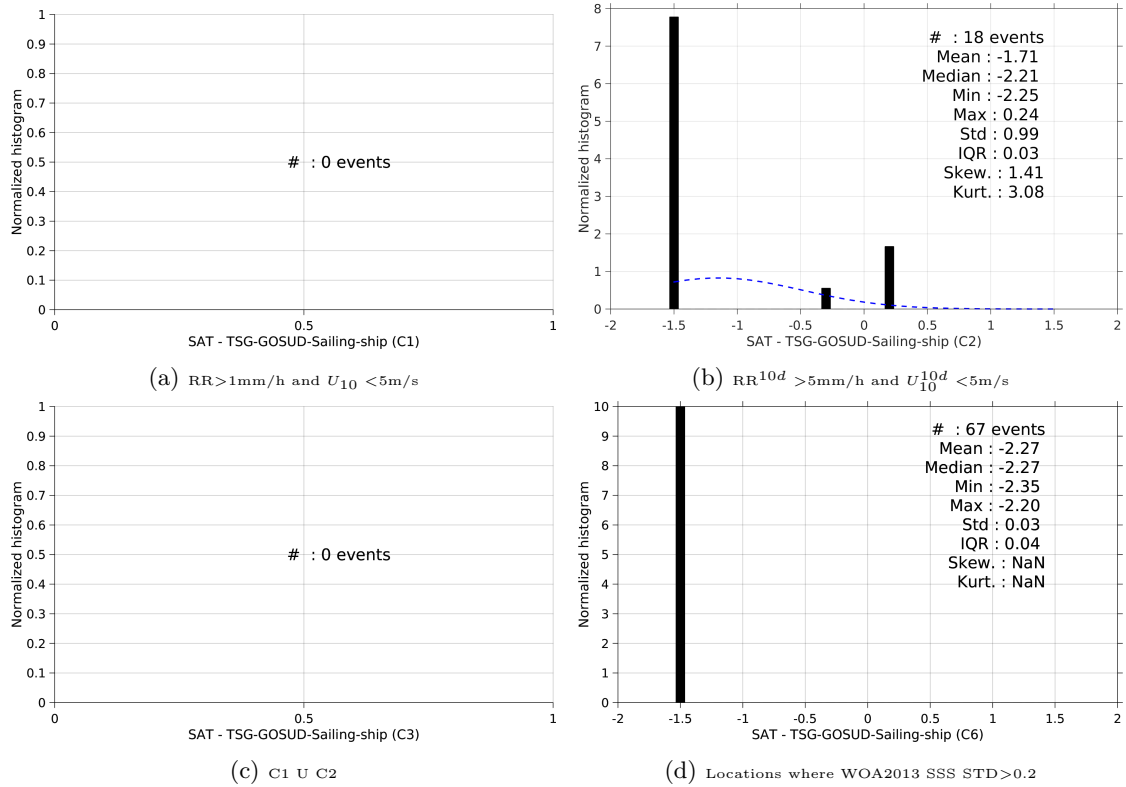
Figure 13: Normalized histogram of \Delta\text{SSS} (Aquarius-L3-OR-V5-7DAY-RUNNING-1DEG - TSG-GOSUD-Sailing-ship) for 6 different subdatasets corresponding to: RR > 1\text{mm/h} and U_{10} < 5\text{m/s} (a), RR^{10d} > 5\text{mm/h} and U_{10}^{10d} < 5\text{m/s} (b), C1 U C2 (c), Locations where WOA2013 SSS STD > 0.2 (d).
