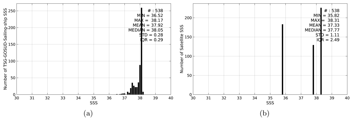
Figure 2: Histograms of SSS from TSG-GOSUD-Sailing-ship (a) and Aquarius-L3-OR-V5-7DAY-RUNNING-1DEG (b) considering all match-up pairs per bins of 0.1 over the Mediterranean Sea Pi-MEP region and for the full satellite product period.
