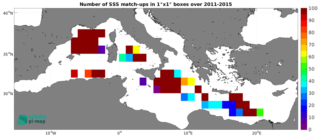
Figure 5: Number of SSS match-ups between TSG (GOSUD-Research-vessel) SSS and the Aquarius SSS L3 OR v5 - 7-Day running (NASA-GSFC) SSS product for the Mediterranean Sea Pi-MEP region over 1^\circ \times 1^\circ boxes and for the full satellite product period.
