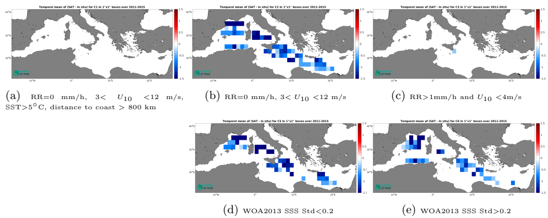
Figure 14: Temporal mean gridded over spatial boxes of size 1^\circ \times 1^\circ of \Delta SSS (Aquarius SSS L3 OR v5 - 7-Day running (NASA-GSFC) - TSG (GOSUD-Research-vessel)) for 5 different subdatasets corresponding to:RR=0 mm/h, 3 < U_{10} < 12 m/s, SST >5^\circ\text{C} , distance to coast > 800 km (a), RR=0 mm/h, 3 < U_{10} < 12 m/s (b), RR >1 mm/h and U_{10} < 4 m/s (c), WOA2013 SSS Std <0.2 (d), WOA2013 SSS Std >0.2 (e).
