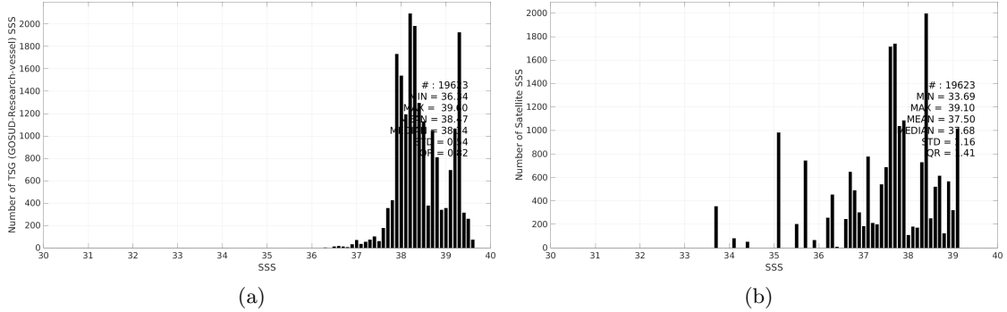
Figure 3: Histograms of SSS from TSG (GOSUD-Research-vessel) (a) and Aquarius SSS L3 OR v5 - 7-Day running (NASA-GSFC) (b) considering all match-up pairs per bins of 0.1 over the Mediterranean Sea Pi-MEP region and for the full satellite product period.
