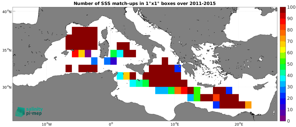
Figure 4: Number of SSS match-ups between TSG (GOSUD-Research-vessel) SSS and the Aquarius SSS L3 OR v5 - 7-Day running (NASA-GSFC) SSS product for the Mediterranean Sea Pi-MEP region over 1^\circ \times 1^\circ boxes and for the full satellite product period.
