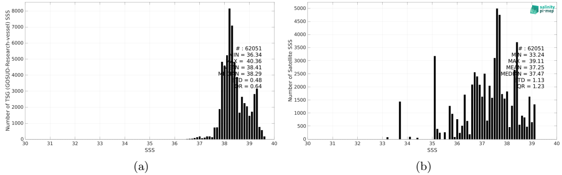
Figure 2: Histograms of SSS from TSG (GOSUD-Research-vessel) (a) and Aquarius SSS L3 OR v5 - 7-Day running (NASA-GSFC) (b) considering all match-up pairs per bins of 0.1 over the Mediterranean Sea Pi-MEP region and for the full satellite product period.
