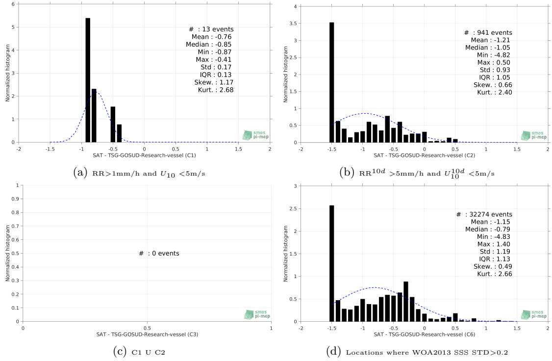
Figure 13: Normalized histogram of \Delta\text{SSS} (Aquarius-L3-OR-V5-7DAY-RUNNING-1DEG - TSG-GOSUD-Research-vessel) for 6 different subdatasets corresponding to: RR > 1mm/h and U_{10} < 5\text{m/s} (a), RR^{10d} > 5\text{mm/h} and U_{10}^{10d} < 5\text{m/s} (b), C1 U C2 (c), Locations where WOA2013 SSS STD > 0.2 (d).
