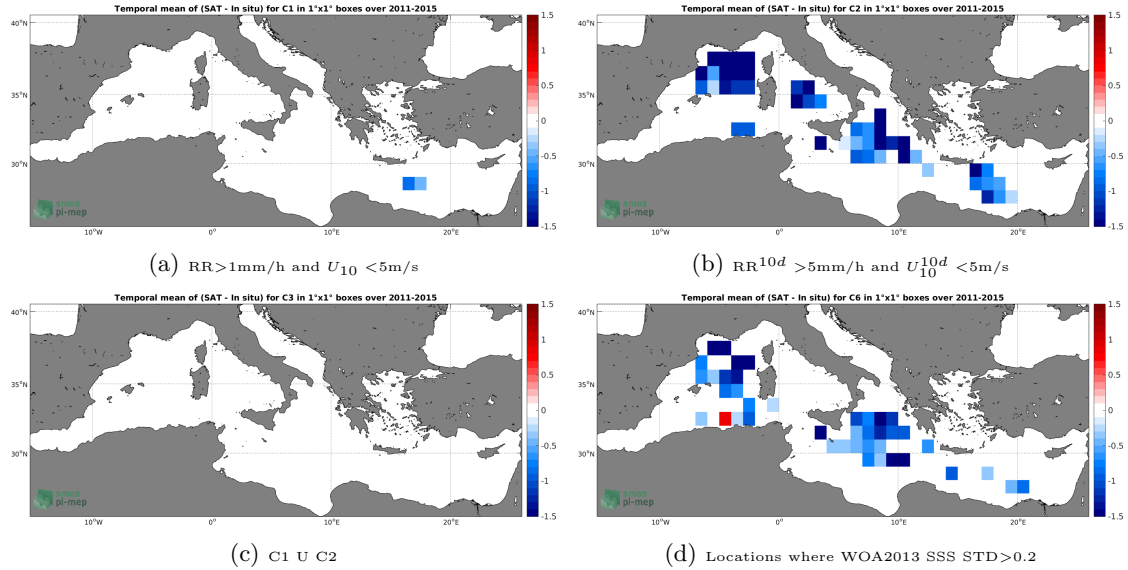
Figure 12: Temporal mean gridded over spatial boxes of size 1^\circ \times 1^\circ of \Delta SSS (Aquarius-L3-OR-V5-7DAY-RUNNING-1DEG - TSG-GOSUD-Research-vessel) for 4 different subdatasets corresponding to: RR > 1\text{mm/h} and U_{10} < 5\text{m/s} (a), RR^{10d} > 5\text{mm/h} and U_{10}^{10d} < 5\text{m/s} (b), C1 U C2 (c), Locations where WOA2013 SSS STD > 0.2 (d).
