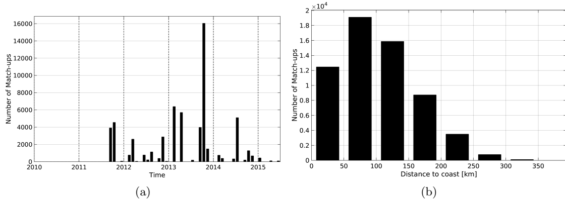
Figure 1: Number of match-ups between TSG-GOSUD-Research-vessel and Aquarius-L3-OR-V5-7DAY-RUNNING-1DEG SSS as a function of time (a) and as function of the distance to coast (b) over the Mediterranean Sea Pi-MEP region and for the full satellite product period.
