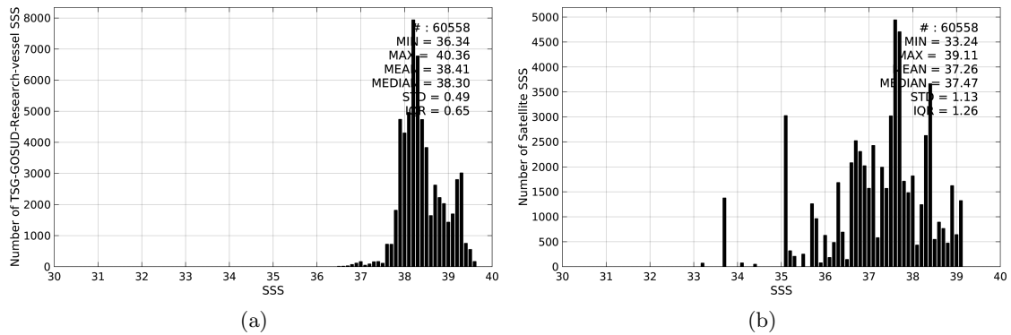
Figure 2: Histograms of SSS from TSG-GOSUD-Research-vessel (a) and Aquarius-L3-OR-V5-7DAY-RUNNING-1DEG (b) considering all match-up pairs per bins of 0.1 over the Mediterranean Sea Pi-MEP region and for the full satellite product period.
