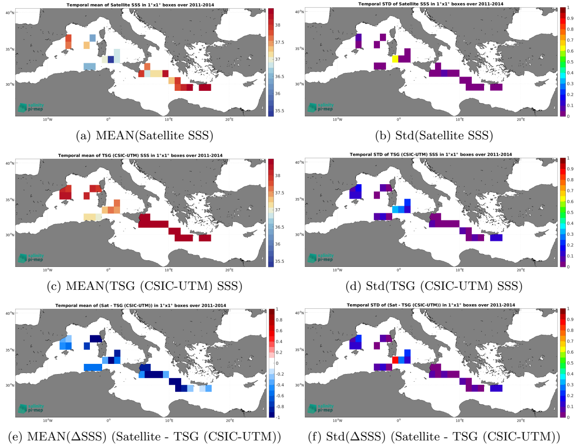
Figure 7: Temporal mean (left) and Std (right) of SSS from Aquarius SSS L3 OR v5 - 7-Day running (NASA-GSFC) (top), TSG (CSIC-UTM) (middle), and of \Delta\text{SSS} (Satellite - TSG (CSIC-UTM)). Only match-up pairs are used to generate these maps.
