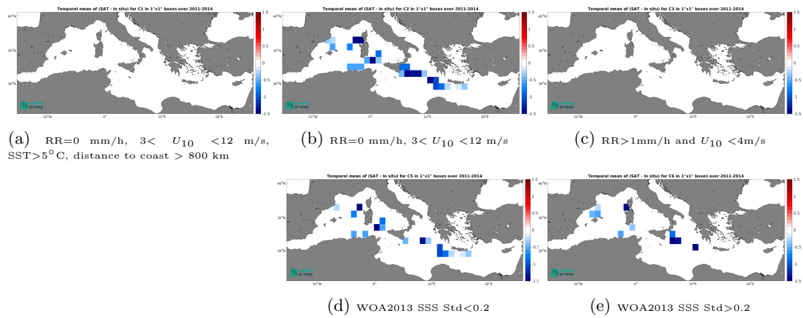
Figure 14: Temporal mean gridded over spatial boxes of size 1^\circ \times 1^\circ of \Delta SSS (Aquarius SSS L3 OR v5 - 7-Day running (NASA-GSFC) - TSG (CSIC-UTM)) for 5 different subdatasets corresponding to:RR=0 mm/h, 3 < U_{10} < 12 m/s, SST >5^\circ\text{C} , distance to coast > 800 km (a), RR=0 mm/h, 3 < U_{10} < 12 m/s (b), RR >1 mm/h and U_{10} < 4 m/s (c), WOA2013 SSS Std <0.2 (d), WOA2013 SSS Std >0.2 (e).
