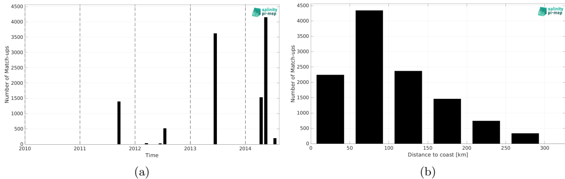
Figure 2: Number of match-ups between TSG (CSIC-UTM) and Aquarius SSS L3 OR v5 - 7-Day running (NASA-GSFC) SSS as a function of time (a) and as function of the distance to coast (b) over the Mediterranean Sea Pi-MEP region and for the full satellite product period.
