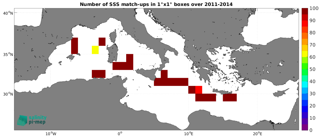
Figure 5: Number of SSS match-ups between TSG (CSIC-UTM) SSS and the Aquarius SSS L3 OR v5 - 7-Day running (NASA-GSFC) SSS product for the Mediterranean Sea Pi-MEP region over 1^\circ \times 1^\circ boxes and for the full satellite product period.
