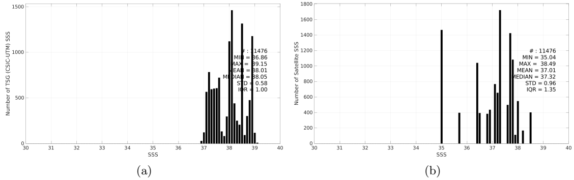
Figure 3: Histograms of SSS from TSG (CSIC-UTM) (a) and Aquarius SSS L3 OR v5 - 7-Day running (NASA-GSFC) (b) considering all match-up pairs per bins of 0.1 over the Mediterranean Sea Pi-MEP region and for the full satellite product period.
