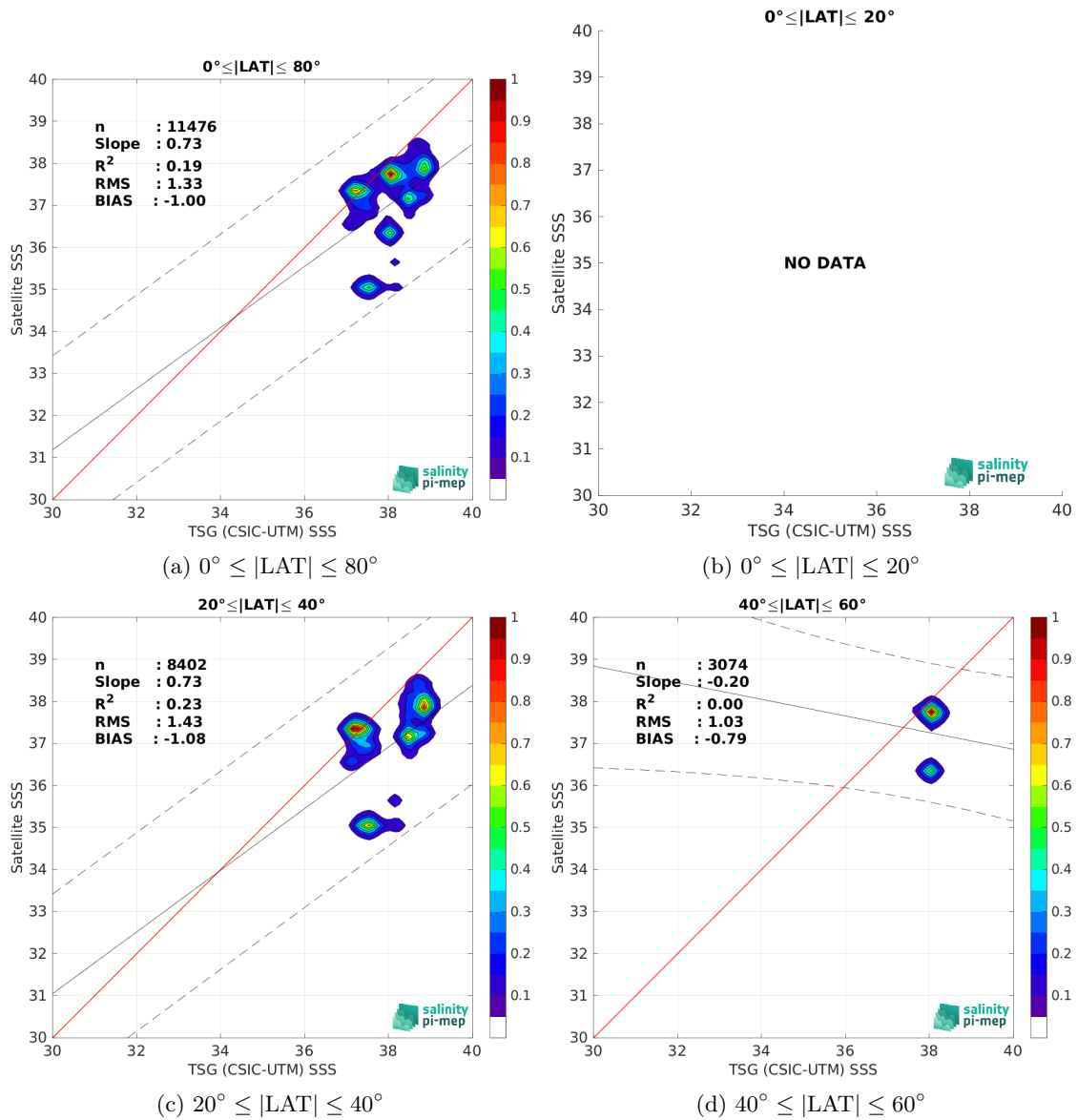
Figure 10: Contour maps of the concentration of Aquarius SSS L3 OR v5 - 7-Day running (NASA-GSFC) SSS (y-axis) versus TSG (CSIC-UTM) SSS (x-axis) at match-up pairs for different latitude bands. For each plot, the red line shows x=y . The black thin and dashed lines indicate a linear fit through the data cloud and the \pm 95\% confidence levels, respectively. The number match-up pairs n , the slope and R^2 coefficient of the linear fit, the root mean square (RMS) and the mean bias between satellite and in situ data are indicated for each latitude band in each plots.
