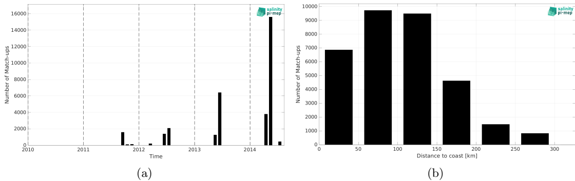
Figure 1: Number of match-ups between TSG (CSIC-UTM) and Aquarius SSS L3 OR v5 - 7-Day running (NASA-GSFC) SSS as a function of time (a) and as function of the distance to coast (b) over the Mediterranean Sea Pi-MEP region and for the full satellite product period.
