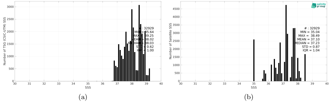
Figure 2: Histograms of SSS from TSG (CSIC-UTM) (a) and Aquarius SSS L3 OR v5 - 7-Day running (NASA-GSFC) (b) considering all match-up pairs per bins of 0.1 over the Mediterranean Sea Pi-MEP region and for the full satellite product period.
