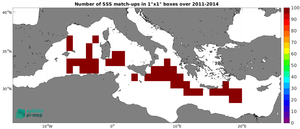
Figure 4: Number of SSS match-ups between TSG (CSIC-UTM) SSS and the Aquarius SSS L3 OR v5 - 7-Day running (NASA-GSFC) SSS product for the Mediterranean Sea Pi-MEP region over 1^\circ \times 1^\circ boxes and for the full satellite product period.
