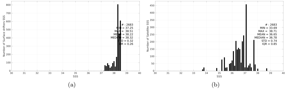
Figure 3: Histograms of SSS from Surface drifters (a) and Aquarius SSS L3 OR v5 - 7-Day running (NASA-GSFC) (b) considering all match-up pairs per bins of 0.1 over the Mediterranean Sea Pi-MEP region and for the full satellite product period.
