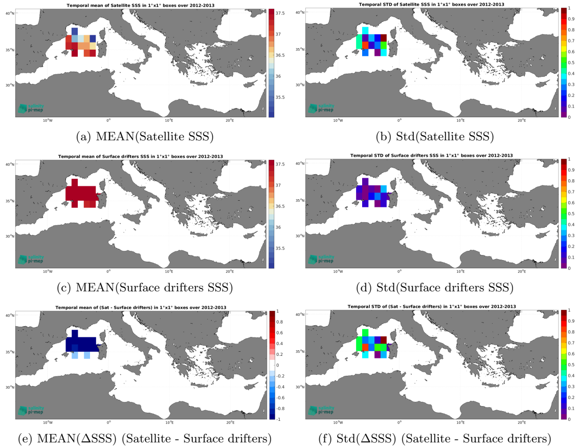
Figure 6: Temporal mean (left) and Std (right) of SSS from Aquarius SSS L3 OR v5 - 7-Day running (NASA-GSFC) (top), Surface drifters (middle), and of \Delta SSS (Satellite - Surface drifters). Only match-up pairs are used to generate these maps.
