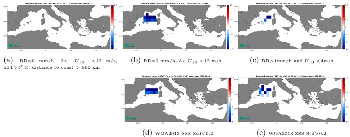
Figure 13: Temporal mean gridded over spatial boxes of size 1^\circ \times 1^\circ of \Delta SSS (Aquarius SSS L3 OR v5 - 7-Day running (NASA-GSFC) - Surface drifters) for 5 different subdatasets corresponding to:RR=0 mm/h, 3 < U_{10} < 12 m/s, SST >5^\circ\text{C} , distance to coast > 800 km (a), RR=0 mm/h, 3 < U_{10} < 12 m/s (b), RR >1 mm/h and U_{10} < 4 m/s (c), WOA2013 SSS Std <0.2 (d), WOA2013 SSS Std >0.2 (e).
