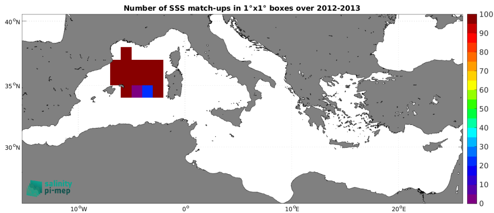
Figure 3: Number of SSS match-ups between Surface drifters SSS and the Aquarius SSS L3 OR v5 - 7-Day running (NASA-GSFC) SSS product for the Mediterranean Sea Pi-MEP region over 1^\circ \times 1^\circ boxes and for the full satellite product period.
