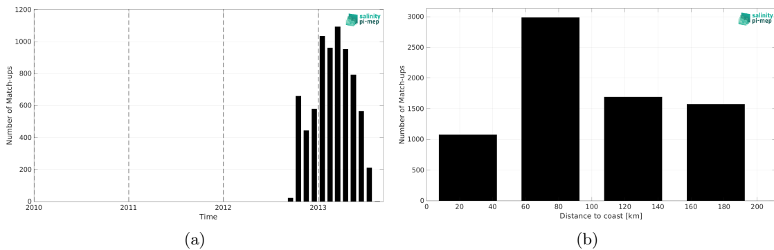
Figure 1: Number of match-ups between Surface drifters and Aquarius SSS L3 OR v5 - 7-Day running (NASA-GSFC) SSS as a function of time (a) and as function of the distance to coast (b) over the Mediterranean Sea Pi-MEP region and for the full satellite product period.
