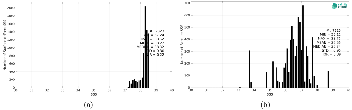
Figure 2: Histograms of SSS from Surface drifters (a) and Aquarius SSS L3 OR v5 - 7-Day running (NASA-GSFC) (b) considering all match-up pairs per bins of 0.1 over the Mediterranean Sea Pi-MEP region and for the full satellite product period.
