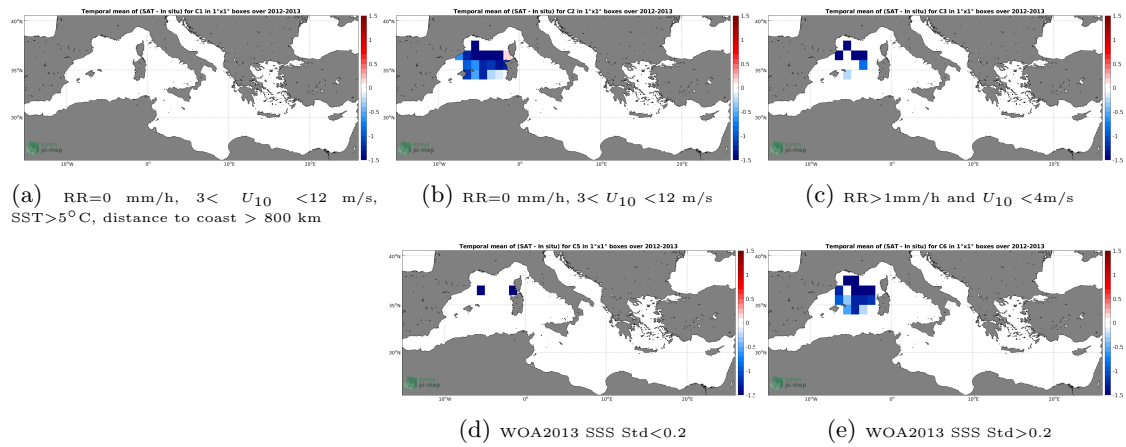
Figure 11: Temporal mean gridded over spatial boxes of size 1^\circ \times 1^\circ of \Delta SSS (Aquarius SSS L3 OR v5 - 7-Day running (NASA-GSFC) - Surface drifters) for 5 different subdatasets corresponding to:RR=0 mm/h, 3 < U_{10} < 12 m/s, SST >5^\circ C, distance to coast > 800 km (a), RR=0 mm/h, 3 < U_{10} < 12 m/s (b), RR >1 mm/h and U_{10} < 4 m/s (c), WOA2013 SSS Std <0.2 (d), WOA2013 SSS Std >0.2 (e).
