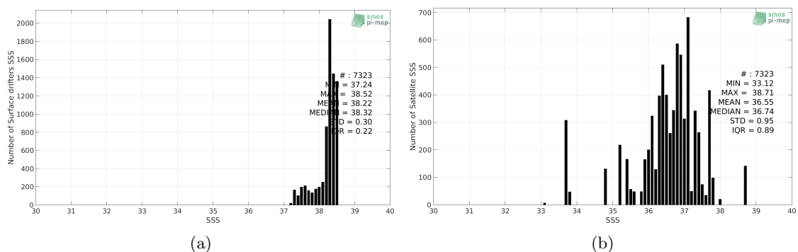
Figure 2: Histograms of SSS from Surface drifters (a) and Aquarius-L3-OR-V5-7DAY-RUNNING-1DEG (b) considering all match-up pairs per bins of 0.1 over the Mediterranean Sea Pi-MEP region and for the full satellite product period.
