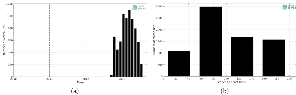
Figure 1: Number of match-ups between Surface drifters and Aquarius-L3-OR-V5-7DAY-RUNNING-1DEG SSS as a function of time (a) and as function of the distance to coast (b) over the Mediterranean Sea Pi-MEP region and for the full satellite product period.
