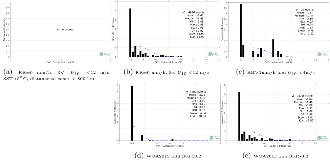
Figure 12: Normalized histogram of \Delta SSS (Aquarius-L3-OR-V5-7DAY-RUNNING-1DEG - Surface drifters) for 5 different subdatasets corresponding to: RR=0 mm/h, 3 < U_{10} < 12 m/s, SST>5°C, distance to coast > 800 km (a), RR=0 mm/h, 3 < U_{10} < 12 m/s (b), RR>1mm/h and U_{10} < 4 m/s (c), WOA2013 SSS Std<0.2 (d), WOA2013 SSS Std>0.2 (e).
