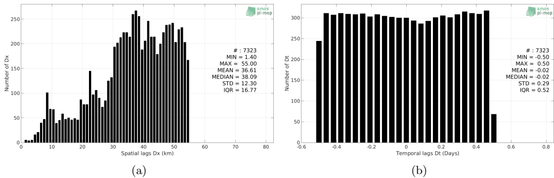
Figure 4: Histograms of the spatial (a) and temporal (b) lags between the time of the Surface drifters measurements and the date of the corresponding Aquarius-L3-OR-V5-7DAY-RUNNING-1DEG SSS product.
