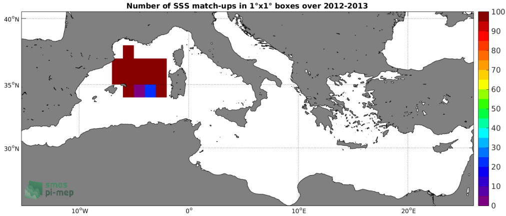
Figure 3: Number of SSS match-ups between Surface drifters SSS and the Aquarius-L3-OR-V5-7DAY-RUNNING-1DEG SSS product for the Mediterranean Sea Pi-MEP region over 1°x1° boxes and for the full satellite product period.
