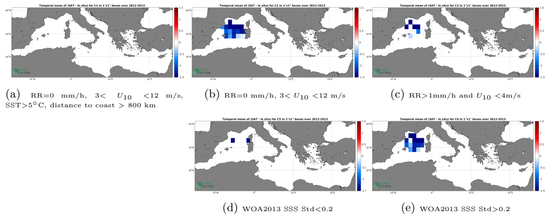
Figure 11: Temporal mean gridded over spatial boxes of size 1^\circ \times 1^\circ of \Delta SSS (Aquarius-L3-OR-V5-7DAY-RUNNING-1DEG - Surface drifters) for 5 different subdatasets corresponding to:RR=0 mm/h, 3 < U_{10} < 12 m/s, SST>5°C, distance to coast > 800 km (a), RR=0 mm/h, 3 < U_{10} < 12 m/s (b), RR>1mm/h and U_{10} < 4 m/s (c), WOA2013 SSS Std<0.2 (d), WOA2013 SSS Std>0.2 (e).
