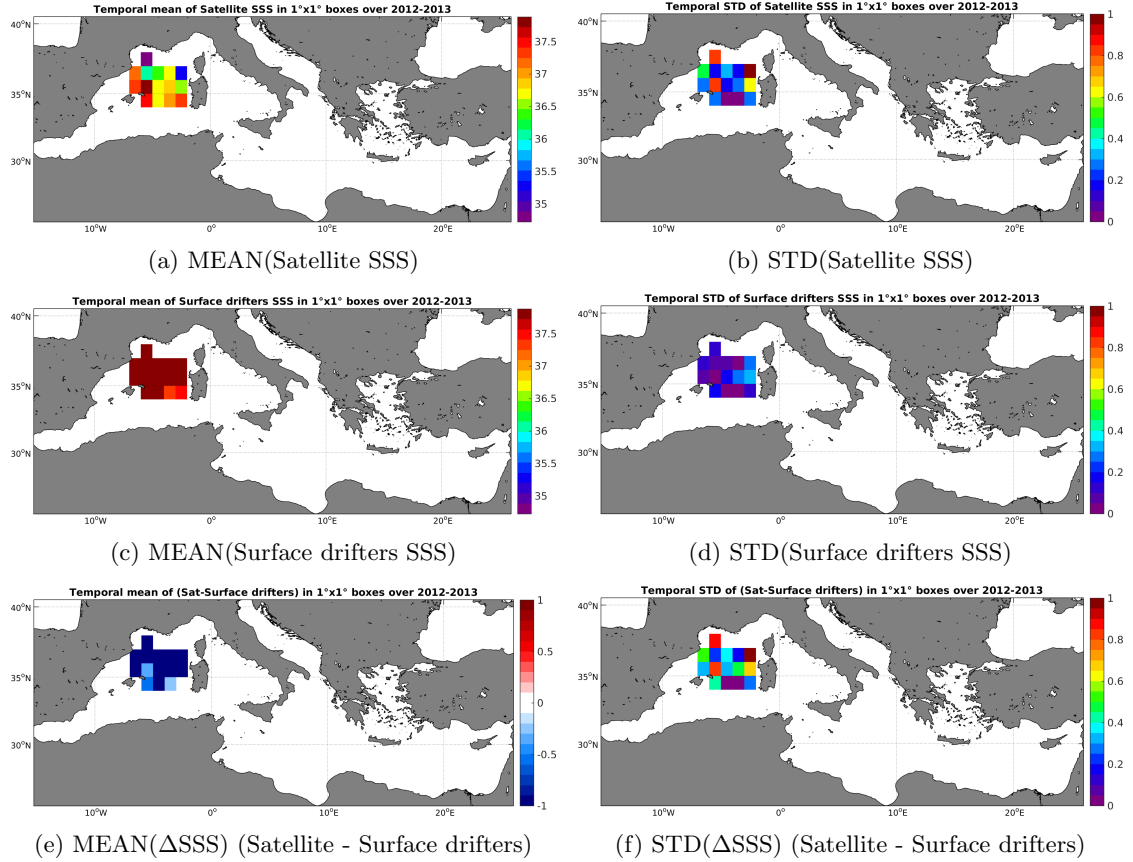
Figure 5: Temporal mean (left) and STD (right) of SSS from Aquarius-L3-OR-V5-7DAY-RUNNING-1DEG (top), Surface drifters (middle), and of \Delta SSS (Satellite - Surface drifters). Only match-up pairs are used to generate these maps.
