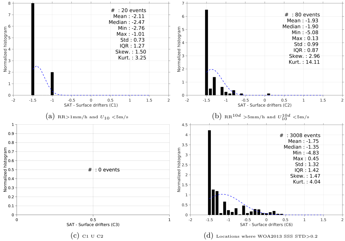
Figure 12: Normalized histogram of \Delta\text{SSS} (Aquarius-L3-OR-V5-7DAY-RUNNING-1DEG - Surface drifters) for 6 different subdatasets corresponding to: RR > 1mm/h and U_{10} < 5\text{m/s} (a), RR^{10d} > 5\text{mm/h} and U_{10}^{10d} < 5\text{m/s} (b), C1 U C2 (c), Locations where WOA2013 SSS STD > 0.2 (d).
