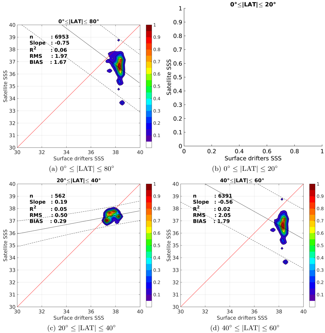
Figure 8: Contour maps of the concentration of Aquarius-L3-OR-V5-7DAY-RUNNING-1DEG SSS (y-axis) versus Surface drifters SSS (x-axis) at match-up pairs for different latitude bands. For each plot, the red line shows x=y . The black thin and dashed lines indicate a linear fit through the data cloud and the \pm 95\% confidence levels, respectively. The number match-up pairs n , the slope and R^2 coefficient of the linear fit, the root mean square (RMS) and the mean bias between satellite and in situ data are indicated for each latitude band in each plots.
