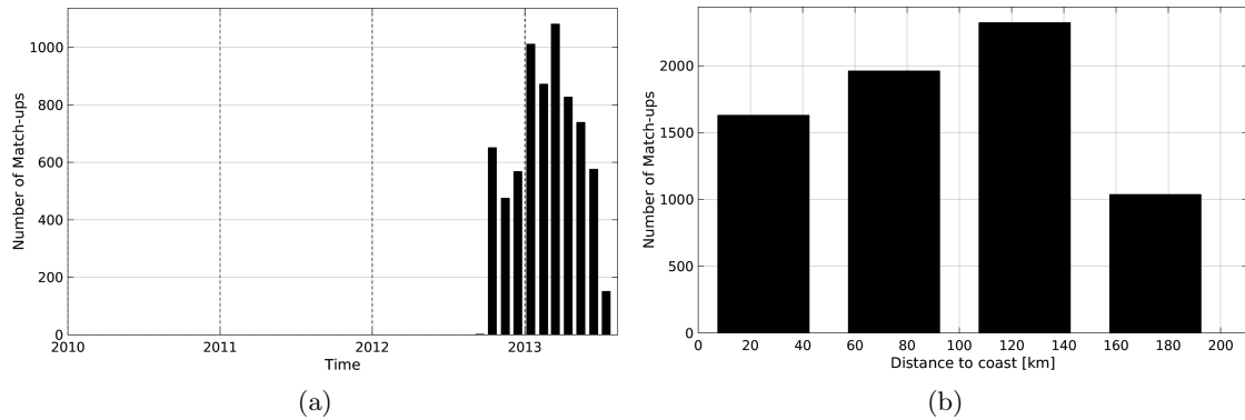
Figure 1: Number of match-ups between Surface drifters and Aquarius-L3-OR-V5-7DAY-RUNNING-1DEG SSS as a function of time (a) and as function of the distance to coast (b) over the Mediterranean Sea Pi-MEP region and for the full satellite product period.
