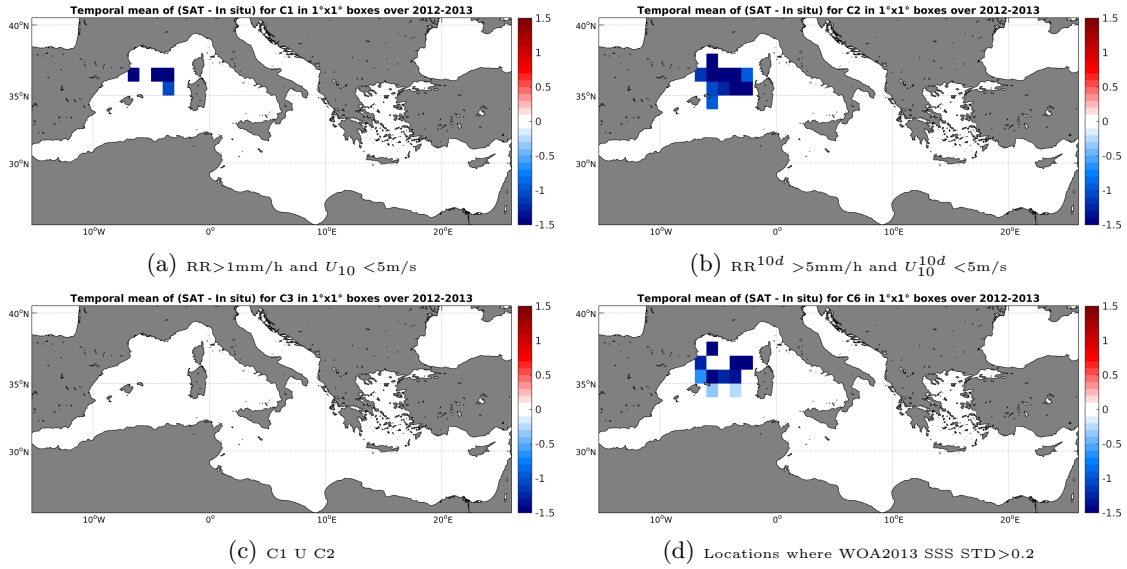
Figure 11: Temporal mean gridded over spatial boxes of size 1°x1° of \Delta SSS (Aquarius-L3-OR-V5-7DAY-RUNNING-1DEG - Surface drifters) for 4 different subdatasets corresponding to: RR > 1\text{mm/h} and U_{10} < 5\text{m/s} (a), RR^{10d} > 5\text{mm/h} and U_{10}^{10d} < 5\text{m/s} (b), C1 U C2 (c), Locations where WOA2013 SSS STD > 0.2 (d).
