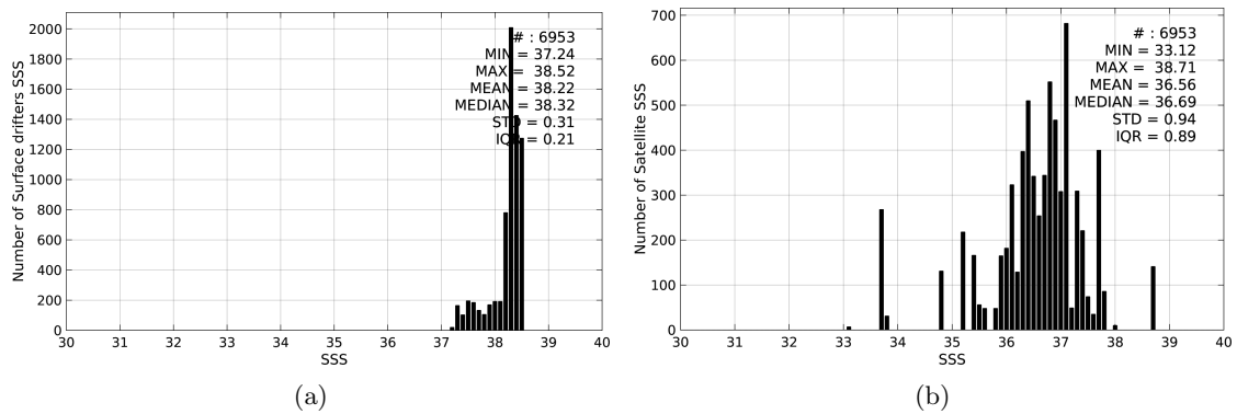
Figure 2: Histograms of SSS from Surface drifters (a) and Aquarius-L3-OR-V5-7DAY-RUNNING-1DEG (b) considering all match-up pairs per bins of 0.1 over the Mediterranean Sea Pi-MEP region and for the full satellite product period.
