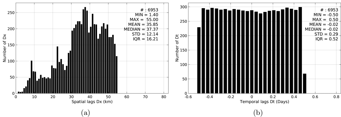
Figure 4: Histograms of the spatial (a) and temporal (b) lags between the time of the Surface drifters measurements and the date of the corresponding Aquarius-L3-OR-V5-7DAY-RUNNING-1DEG SSS product.
