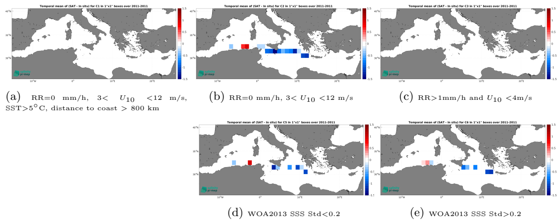
Figure 14: Temporal mean gridded over spatial boxes of size 1^\circ \times 1^\circ of \Delta SSS (Aquarius SSS L3 OR v5 - 7-Day running - Rain mask (NASA-GSFC) - TSG (SAMOS)) for 5 different subdatasets corresponding to:RR=0 mm/h, 3 < U_{10} < 12 m/s, SST>5°C, distance to coast > 800 km (a), RR=0 mm/h, 3 < U_{10} < 12 m/s (b), RR>1mm/h and U_{10} < 4 m/s (c), WOA2013 SSS Std<0.2 (d), WOA2013 SSS Std>0.2 (e).
