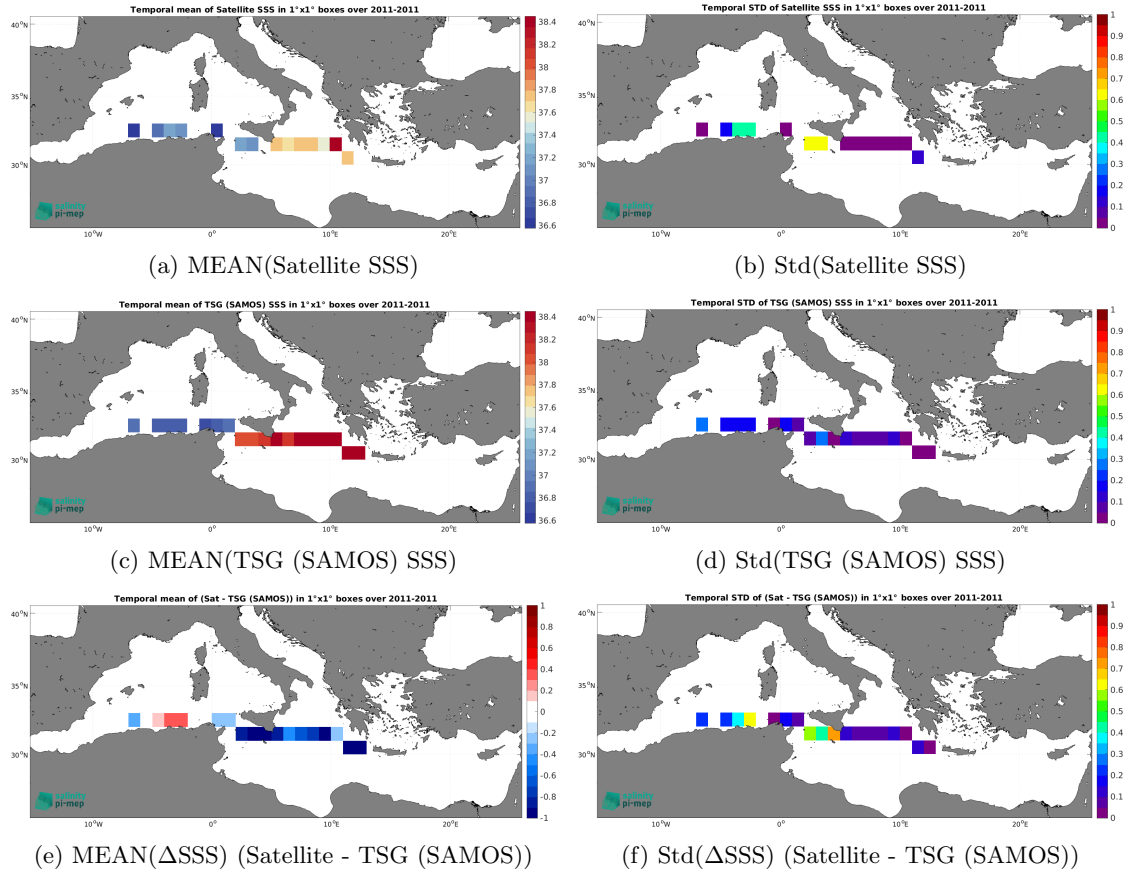
Figure 7: Temporal mean (left) and Std (right) of SSS from Aquarius SSS L3 OR v5 - 7-Day running - Rain mask (NASA-GSFC) (top), TSG (SAMOS) (middle), and of \Delta\text{SSS} (Satellite - TSG (SAMOS)). Only match-up pairs are used to generate these maps.
