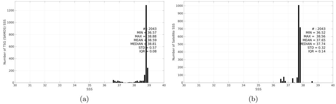
Figure 3: Histograms of SSS from TSG (SAMOS) (a) and Aquarius SSS L3 OR v5 - 7-Day running - Rain mask (NASA-GSFC) (b) considering all match-up pairs per bins of 0.1 over the Mediterranean Sea Pi-MEP region and for the full satellite product period.
