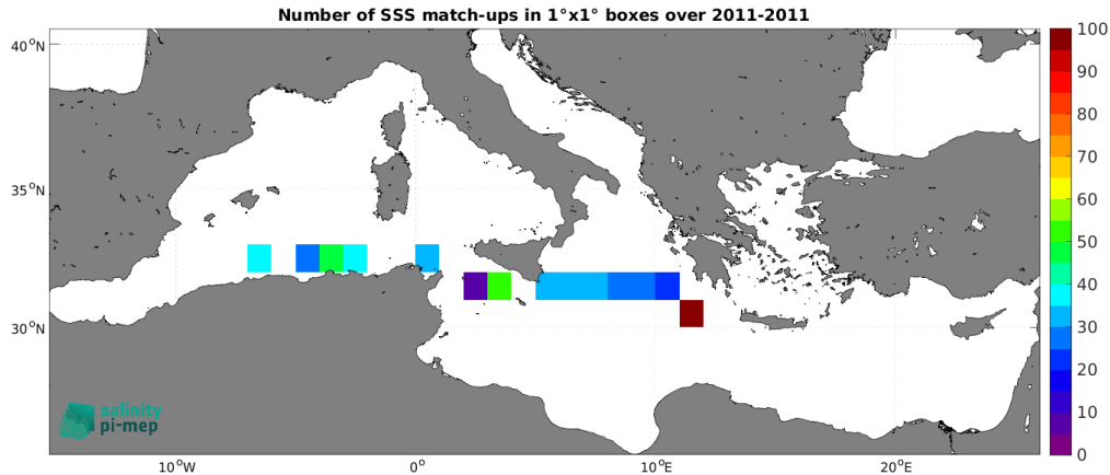
Figure 5: Number of SSS match-ups between TSG (SAMOS) SSS and the Aquarius SSS L3 OR v5 - 7-Day running - Rain mask (NASA-GSFC) SSS product for the Mediterranean Sea Pi-MEP region over 1^\circ \times 1^\circ boxes and for the full satellite product period.
