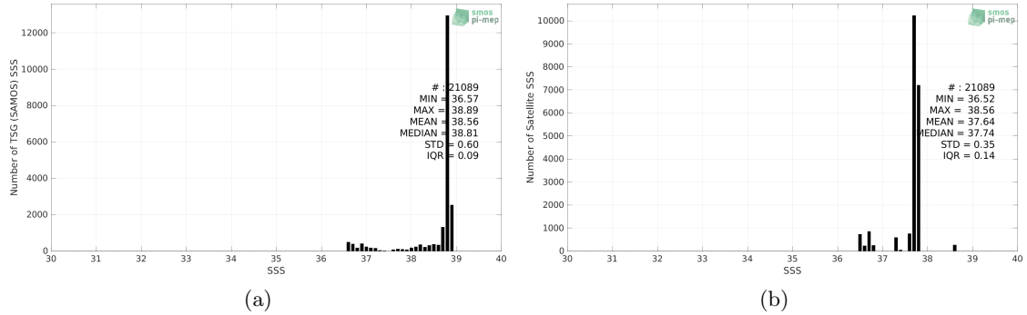
Figure 2: Histograms of SSS from TSG (SAMOS) (a) and Aquarius SSS L3 OR v5 - 7-Day running - Rain mask (NASA-GSFC) (b) considering all match-up pairs per bins of 0.1 over the Mediterranean Sea Pi-MEP region and for the full satellite product period.
