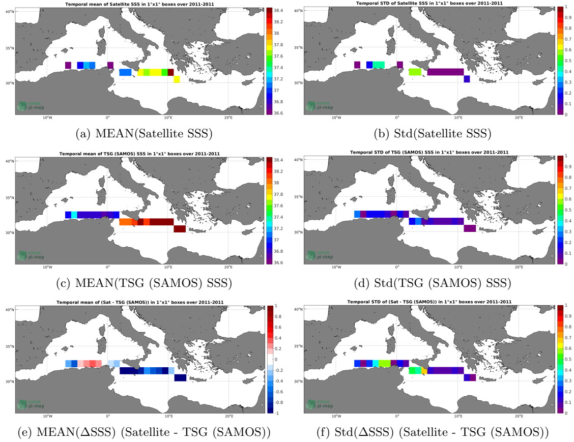
Figure 6: Temporal mean (left) and Std (right) of SSS from Aquarius SSS L3 OR v5 - 7-Day running - Rain mask (NASA-GSFC) (top), TSG (SAMOS) (middle), and of \Delta SSS (Satellite - TSG (SAMOS)). Only match-up pairs are used to generate these maps.
