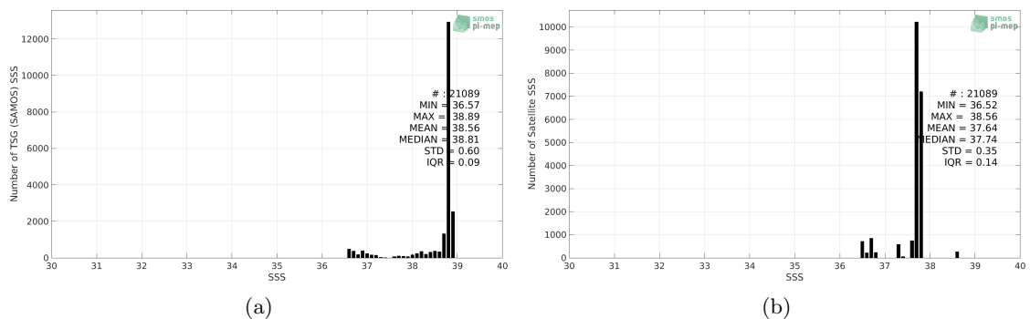
Figure 2: Histograms of SSS from TSG (SAMOS) (a) and Aquarius SSS L3 OR v5 - 7-Day running - Rain mask (NASA-GSFC) (b) considering all match-up pairs per bins of 0.1 over the Mediterranean Sea Pi-MEP region and for the full satellite product period.
