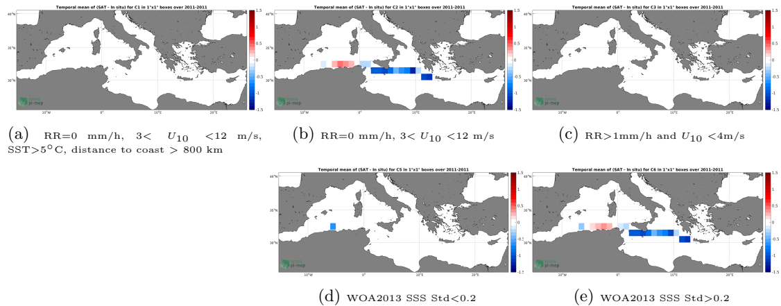
Figure 12: Temporal mean gridded over spatial boxes of size 1^{\circ}\times 1^{\circ} of \Delta\text{SSS} (Aquarius-L3-OR-V5-7DAY-RUNNING-RAIN-MASK-1DEG - TSG-SAMOS) for 5 different subdatasets corresponding to:RR=0 mm/h, 3 < U_{10} < 12 m/s, SST > 5^{\circ}\text{C} , distance to coast > 800 km (a), RR=0 mm/h, 3 < U_{10} < 12 m/s (b), RR > 1 mm/h and U_{10} < 4 m/s (c), WOA2013 SSS Std < 0.2 (d), WOA2013 SSS Std > 0.2 (e).
