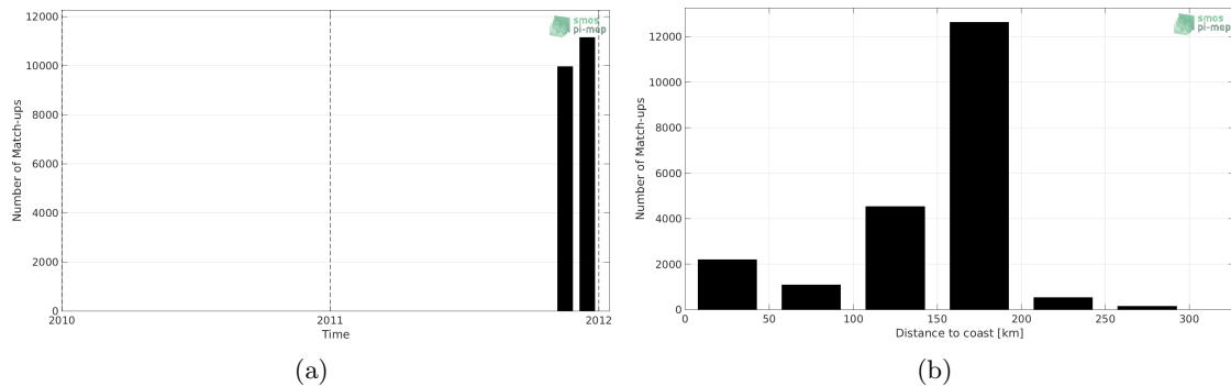
Figure 1: Number of match-ups between TSG-SAMOS and Aquarius-L3-OR-V5-7DAY-RUNNING-RAIN-MASK-1DEG SSS as a function of time (a) and as function of the distance to coast (b) over the Mediterranean Sea Pi-MEP region and for the full satellite product period.
