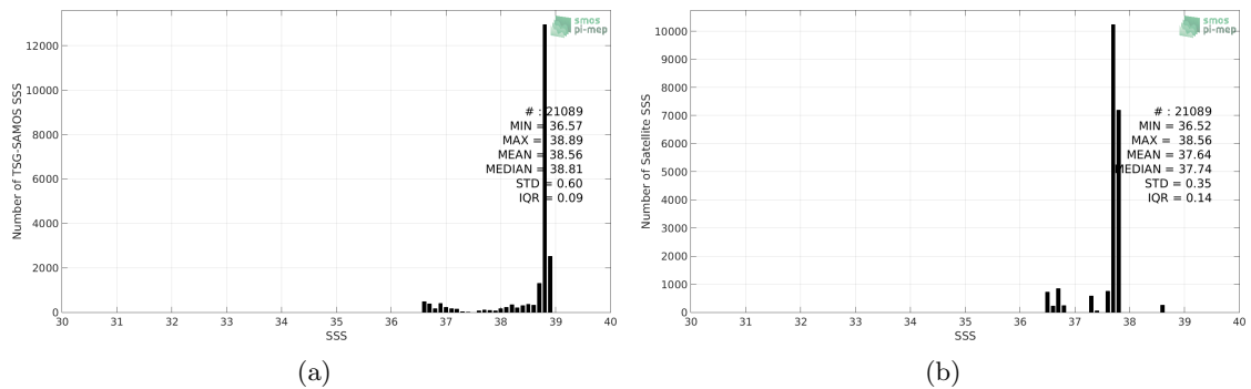
Figure 2: Histograms of SSS from TSG-SAMOS (a) and Aquarius-L3-OR-V5-7DAY-RUNNING-RAIN-MASK-1DEG (b) considering all match-up pairs per bins of 0.1 over the Mediterranean Sea Pi-MEP region and for the full satellite product period.
