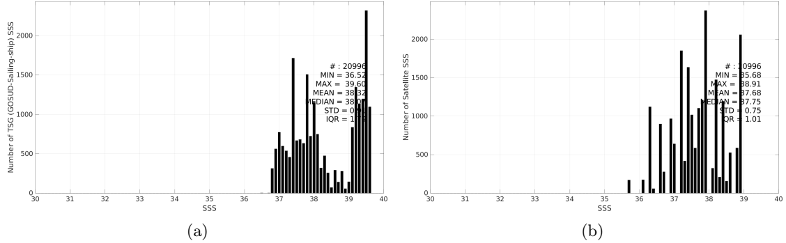
Figure 3: Histograms of SSS from TSG (GOSUD-Sailing-ship) (a) and Aquarius SSS L3 OR v5 - 7-Day running - Rain mask (NASA-GSFC) (b) considering all match-up pairs per bins of 0.1 over the Mediterranean Sea Pi-MEP region and for the full satellite product period.
