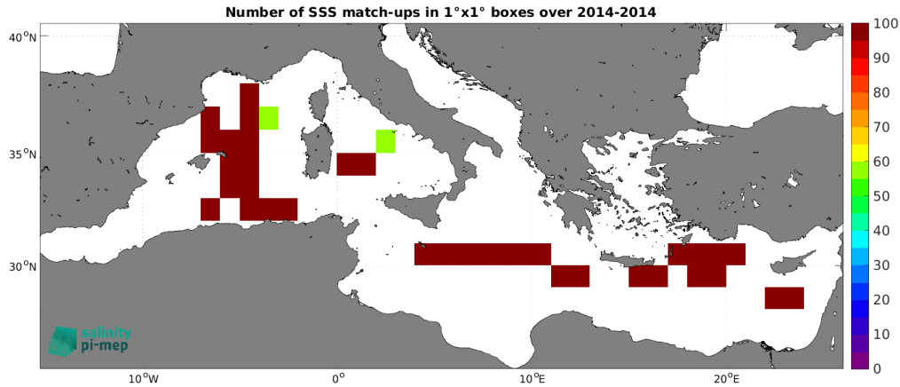
Figure 5: Number of SSS match-ups between TSG (GOSUD-Sailing-ship) SSS and the Aquarius SSS L3 OR v5 - 7-Day running - Rain mask (NASA-GSFC) SSS product for the Mediterranean Sea Pi-MEP region over 1^\circ \times 1^\circ boxes and for the full satellite product period.
