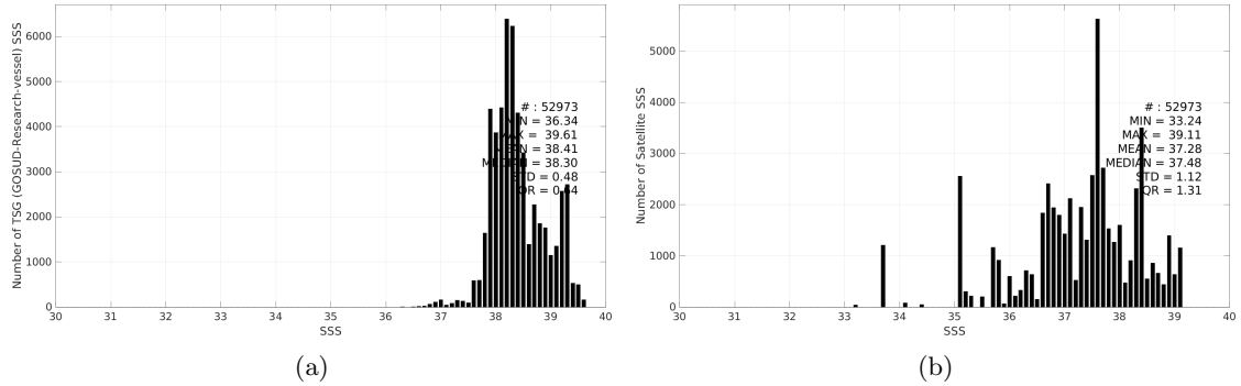
Figure 3: Histograms of SSS from TSG (GOSUD-Research-vessel) (a) and Aquarius SSS L3 OR v5 - 7-Day running - Rain mask (NASA-GSFC) (b) considering all match-up pairs per bins of 0.1 over the Mediterranean Sea Pi-MEP region and for the full satellite product period.
