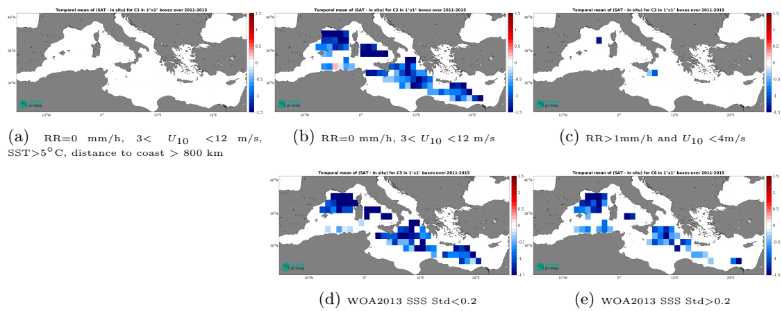
Figure 14: Temporal mean gridded over spatial boxes of size 1^\circ \times 1^\circ of \Delta\text{SSS} (Aquarius SSS L3 OR v5 - 7-Day running - Rain mask (NASA-GSFC) - TSG (GOSUD-Research-vessel)) for 5 different subdatasets corresponding to:RR=0 mm/h, 3 < U_{10} < 12 m/s, SST >5^\circ\text{C} , distance to coast > 800 km (a), RR=0 mm/h, 3 < U_{10} < 12 m/s (b), RR >1 mm/h and U_{10} < 4 m/s (c), WOA2013 SSS Std <0.2 (d), WOA2013 SSS Std >0.2 (e).
