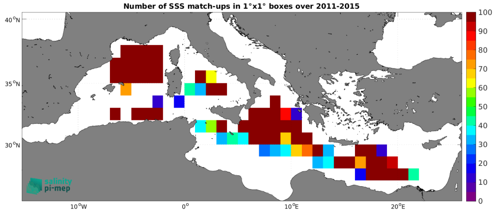
Figure 5: Number of SSS match-ups between TSG (GOSUD-Research-vessel) SSS and the Aquarius SSS L3 OR v5 - 7-Day running - Rain mask (NASA-GSFC) SSS product for the Mediterranean Sea Pi-MEP region over 1^\circ \times 1^\circ boxes and for the full satellite product period.
