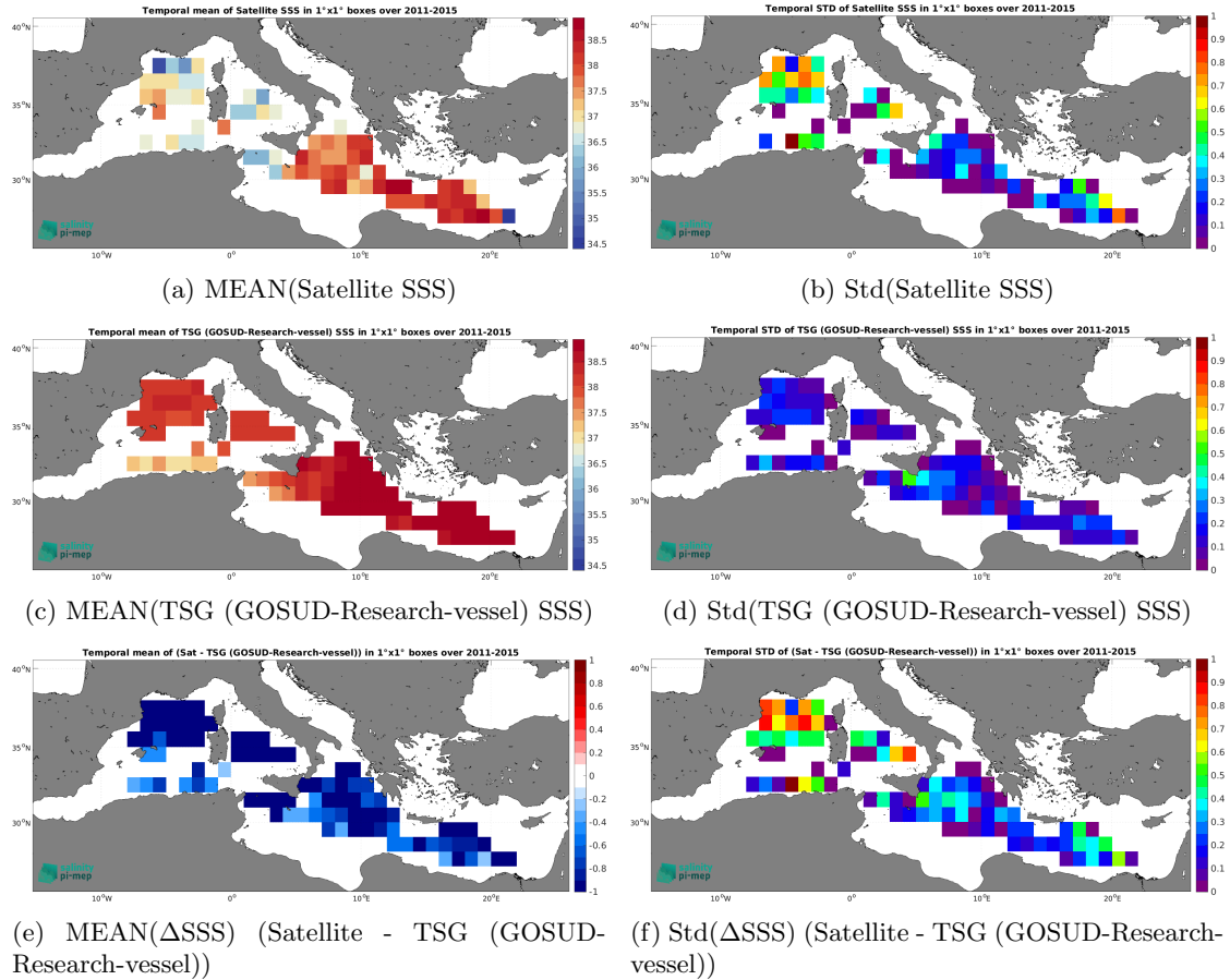
Figure 7: Temporal mean (left) and Std (right) of SSS from Aquarius SSS L3 OR v5 - 7-Day running - Rain mask (NASA-GSFC) (top), TSG (GOSUD-Research-vessel) (middle), and of \Delta\text{SSS} (Satellite - TSG (GOSUD-Research-vessel)). Only match-up pairs are used to generate these maps.
