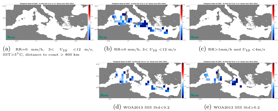
Figure 14: Temporal mean gridded over spatial boxes of size 1^\circ \times 1^\circ of \Delta SSS (Aquarius SSS L3 OR v5 - 7-Day running - Rain mask (NASA-GSFC) - TSG (CSIC-UTM)) for 5 different subdatasets corresponding to:RR=0 mm/h, 3 < U_{10} < 12 m/s, SST >5^\circ\text{C} , distance to coast > 800 km (a), RR=0 mm/h, 3 < U_{10} < 12 m/s (b), RR >1 mm/h and U_{10} < 4 m/s (c), WOA2013 SSS Std <0.2 (d), WOA2013 SSS Std >0.2 (e).
