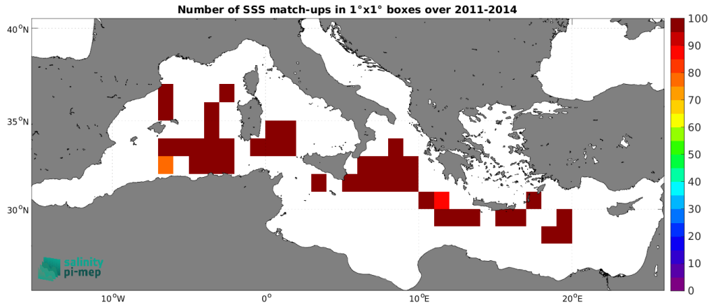
Figure 5: Number of SSS match-ups between TSG (CSIC-UTM) SSS and the Aquarius SSS L3 OR v5 - 7-Day running - Rain mask (NASA-GSFC) SSS product for the Mediterranean Sea Pi-MEP region over 1^\circ \times 1^\circ boxes and for the full satellite product period.
