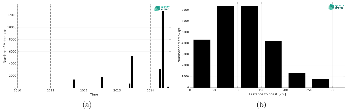
Figure 2: Number of match-ups between TSG (CSIC-UTM) and Aquarius SSS L3 OR v5 - 7-Day running - Rain mask (NASA-GSFC) SSS as a function of time (a) and as function of the distance to coast (b) over the Mediterranean Sea Pi-MEP region and for the full satellite product period.
