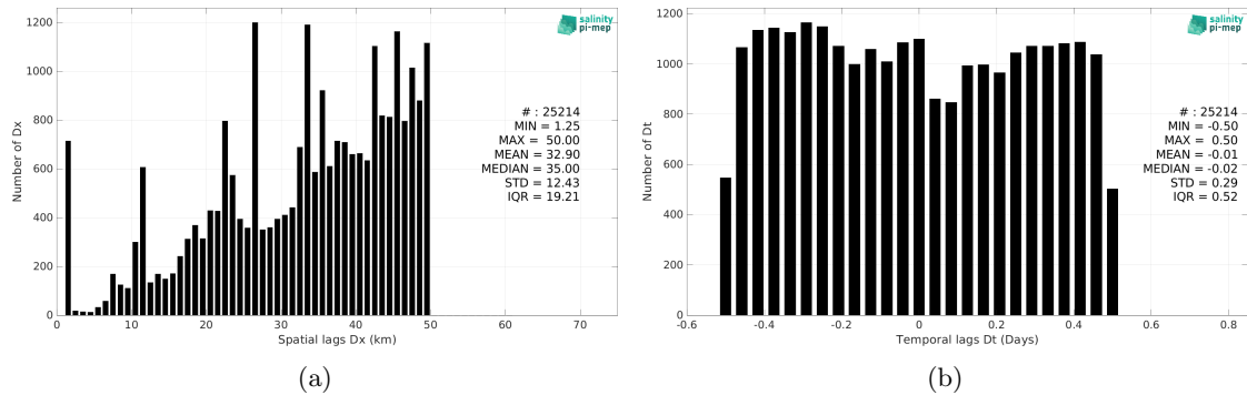
Figure 6: Histograms of the spatial (a) and temporal (b) lags between the location/time of the TSG (CSIC-UTM) measurement and the date of the corresponding Aquarius SSS L3 OR v5 - 7-Day running - Rain mask (NASA-GSFC) SSS pixel.
