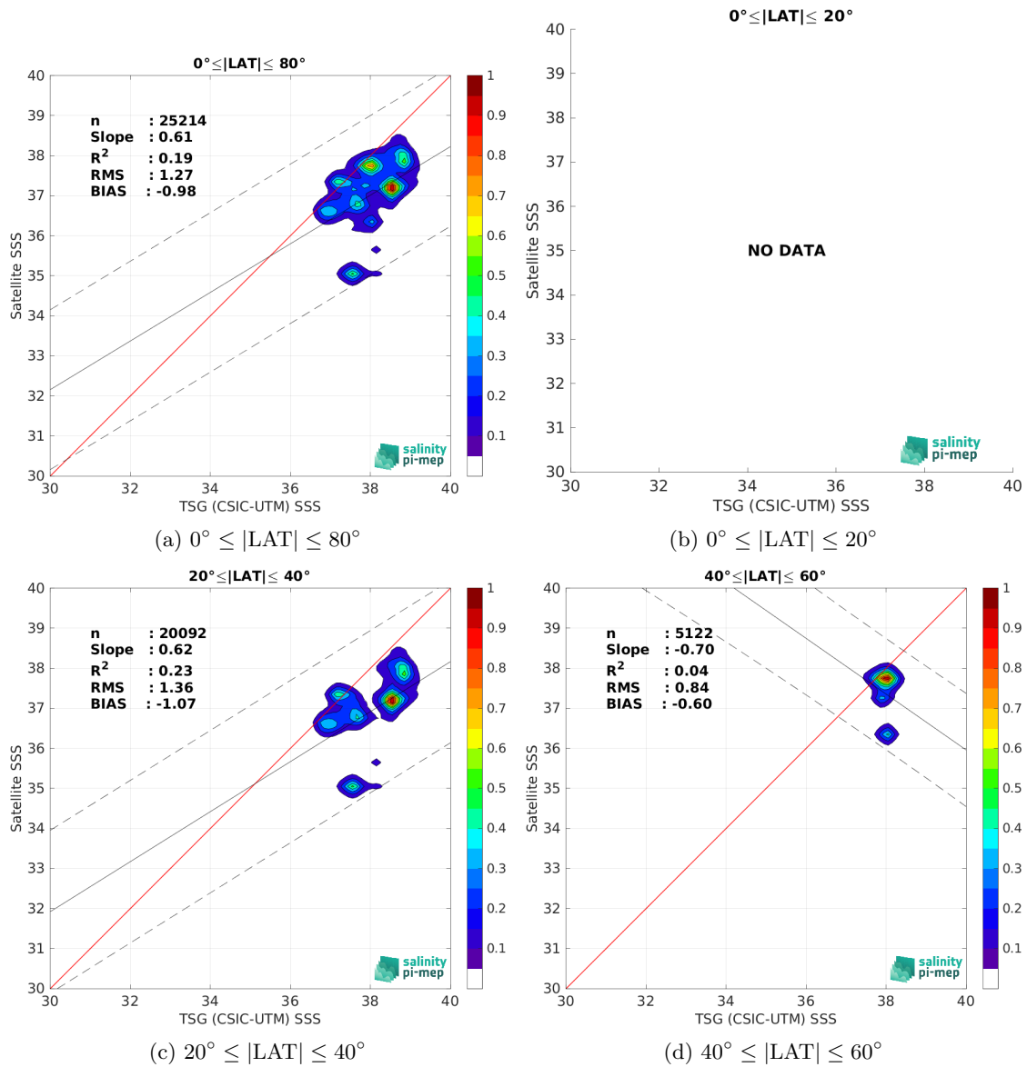
Figure 10: Contour maps of the concentration of Aquarius SSS L3 OR v5 - 7-Day running - Rain mask (NASA-GSFC) SSS (y-axis) versus TSG (CSIC-UTM) SSS (x-axis) at match-up pairs for different latitude bands. For each plot, the red line shows x=y . The black thin and dashed lines indicate a linear fit through the data cloud and the \pm 95\% confidence levels, respectively. The number match-up pairs n , the slope and R^2 coefficient of the linear fit, the root mean square (RMS) and the mean bias between satellite and in situ data are indicated for each latitude band in each plots.
