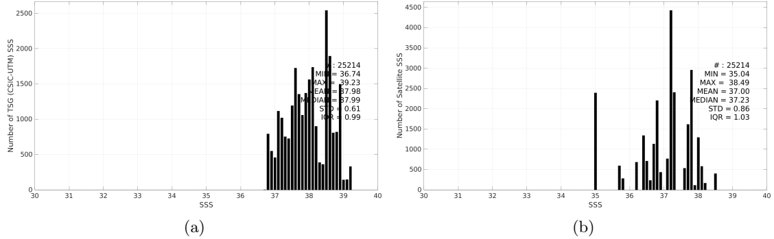
Figure 3: Histograms of SSS from TSG (CSIC-UTM) (a) and Aquarius SSS L3 OR v5 - 7-Day running - Rain mask (NASA-GSFC) (b) considering all match-up pairs per bins of 0.1 over the Mediterranean Sea Pi-MEP region and for the full satellite product period.
