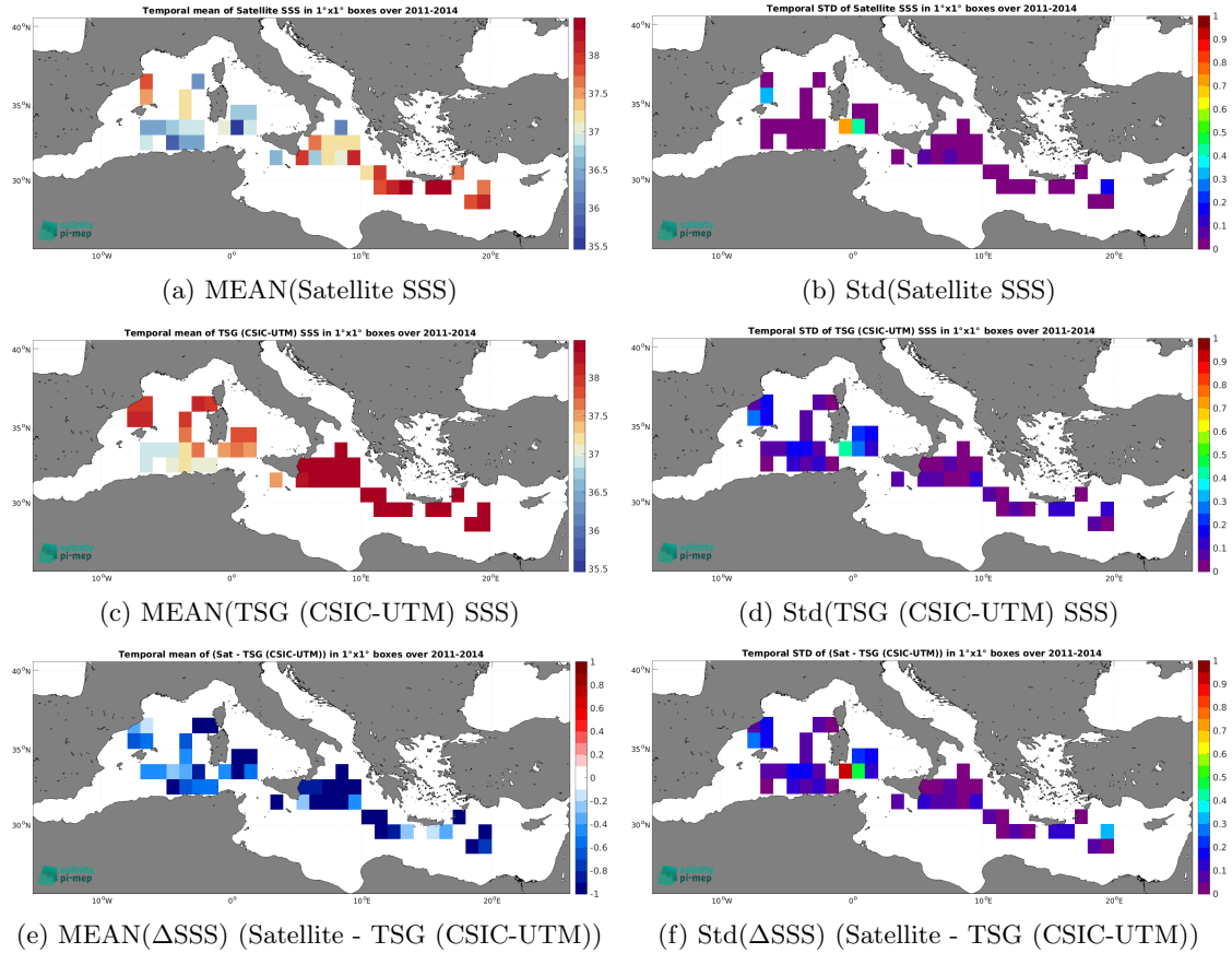
Figure 7: Temporal mean (left) and Std (right) of SSS from Aquarius SSS L3 OR v5 - 7-Day running - Rain mask (NASA-GSFC) (top), TSG (CSIC-UTM) (middle), and of \Delta\text{SSS} (Satellite - TSG (CSIC-UTM)). Only match-up pairs are used to generate these maps.
