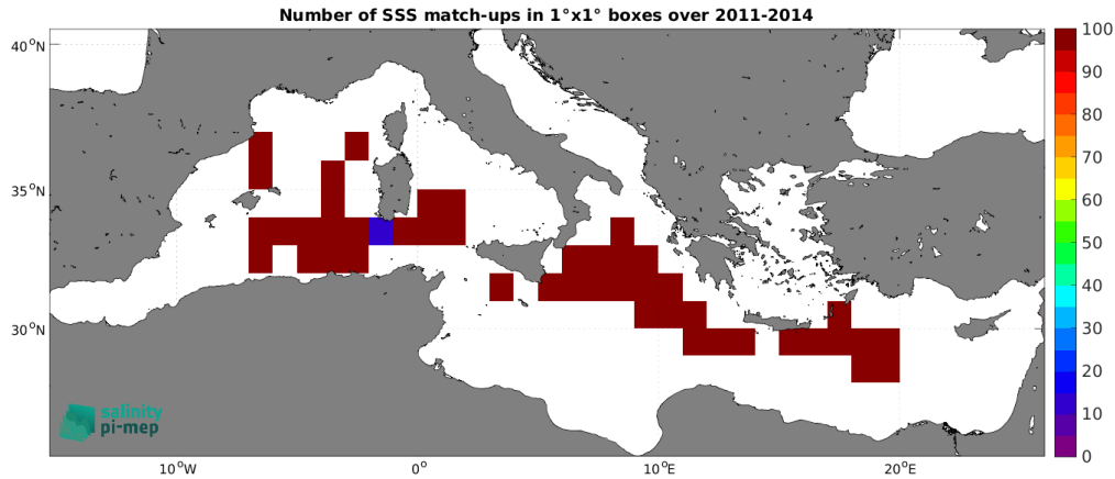
Figure 4: Number of SSS match-ups between TSG (CSIC-UTM) SSS and the Aquarius SSS L3 OR v5 - 7-Day running - Rain mask (NASA-GSFC) SSS product for the Mediterranean Sea Pi-MEP region over 1^\circ \times 1^\circ boxes and for the full satellite product period.
