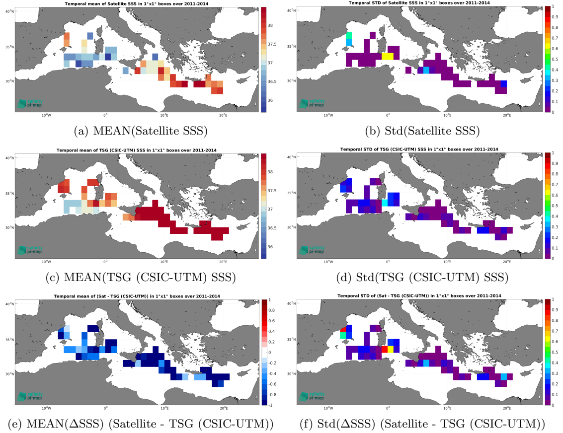
Figure 6: Temporal mean (left) and Std (right) of SSS from Aquarius SSS L3 OR v5 - 7-Day running - Rain mask (NASA-GSFC) (top), TSG (CSIC-UTM) (middle), and of \Delta\text{SSS} (Satellite - TSG (CSIC-UTM)). Only match-up pairs are used to generate these maps.
