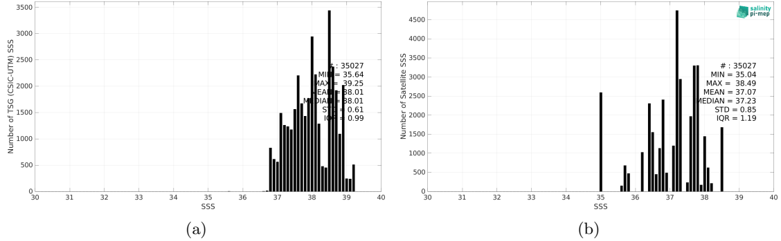
Figure 2: Histograms of SSS from TSG (CSIC-UTM) (a) and Aquarius SSS L3 OR v5 - 7-Day running - Rain mask (NASA-GSFC) (b) considering all match-up pairs per bins of 0.1 over the Mediterranean Sea Pi-MEP region and for the full satellite product period.
