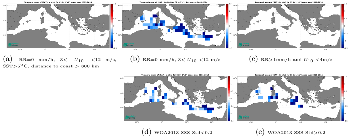
Figure 12: Temporal mean gridded over spatial boxes of size 1^{\circ}\times 1^{\circ} of \Delta\text{SSS} (Aquarius SSS L3 OR v5 - 7-Day running - Rain mask (NASA-GSFC) - TSG (CSIC-UTM)) for 5 different subdatasets corresponding to:RR=0 mm/h, 3 < U_{10} < 12 m/s, SST >5^{\circ}\text{C} , distance to coast > 800 km (a), RR=0 mm/h, 3 < U_{10} < 12 m/s (b), RR >1 mm/h and U_{10} < 4 m/s (c), WOA2013 SSS Std <0.2 (d), WOA2013 SSS Std >0.2 (e).
