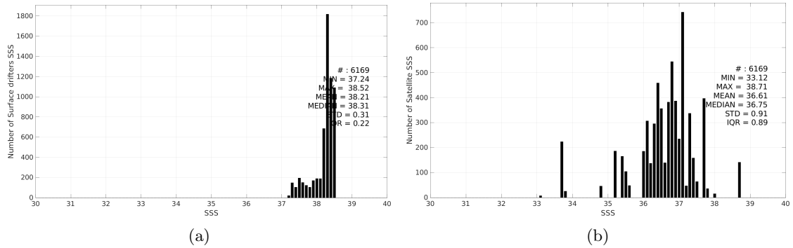
Figure 3: Histograms of SSS from Surface drifters (a) and Aquarius SSS L3 OR v5 - 7-Day running - Rain mask (NASA-GSFC) (b) considering all match-up pairs per bins of 0.1 over the Mediterranean Sea Pi-MEP region and for the full satellite product period.
