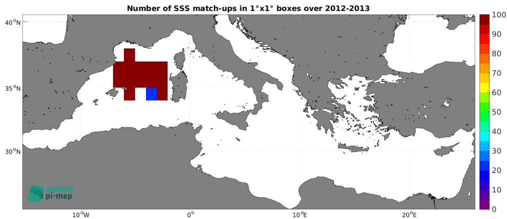
Figure 4: Number of SSS match-ups between Surface drifters SSS and the Aquarius SSS L3 OR v5 - 7-Day running - Rain mask (NASA-GSFC) SSS product for the Mediterranean Sea Pi-MEP region over 1^\circ \times 1^\circ boxes and for the full satellite product period.
