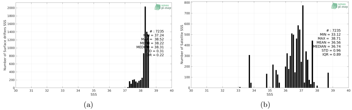
Figure 2: Histograms of SSS from Surface drifters (a) and Aquarius SSS L3 OR v5 - 7-Day running - Rain mask (NASA-GSFC) (b) considering all match-up pairs per bins of 0.1 over the Mediterranean Sea Pi-MEP region and for the full satellite product period.
