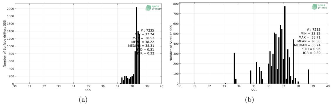
Figure 2: Histograms of SSS from Surface drifters (a) and Aquarius-L3-OR-V5-7DAY-RUNNING-RAIN-MASK-1DEG (b) considering all match-up pairs per bins of 0.1 over the Mediterranean Sea Pi-MEP region and for the full satellite product period.
