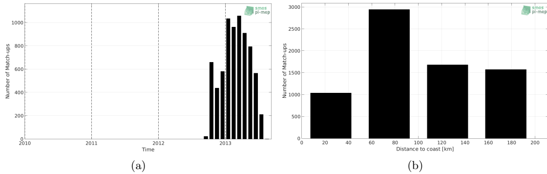
Figure 1: Number of match-ups between Surface drifters and Aquarius-L3-OR-V5-7DAY-RUNNING-RAIN-MASK-1DEG SSS as a function of time (a) and as function of the distance to coast (b) over the Mediterranean Sea Pi-MEP region and for the full satellite product period.
