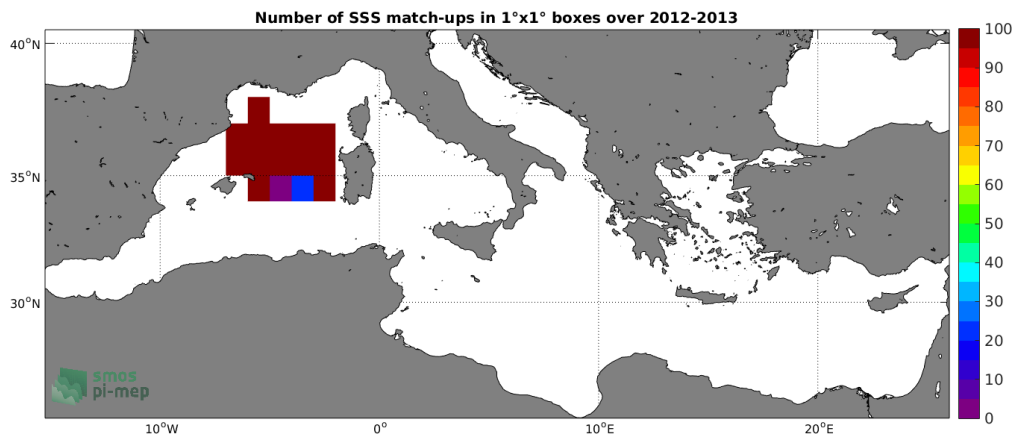
Figure 3: Number of SSS match-ups between Surface drifters SSS and the Aquarius-L3-OR-V5-7DAY-RUNNING-RAIN-MASK-1DEG SSS product for the Mediterranean Sea Pi-MEP region over 1°x1° boxes and for the full satellite product period.
