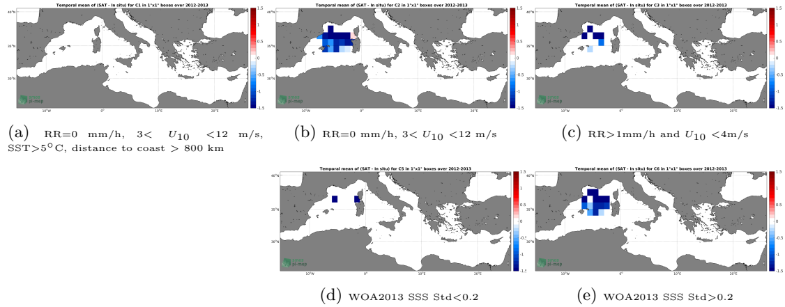
Figure 11: Temporal mean gridded over spatial boxes of size 1^{\circ}\times 1^{\circ} of \Delta\text{SSS} (Aquarius-L3-OR-V5-7DAY-RUNNING-RAIN-MASK-1DEG - Surface drifters) for 5 different subdatasets corresponding to:RR=0 mm/h, 3 < U_{10} < 12 m/s, SST > 5^{\circ}\text{C} , distance to coast > 800 km (a), RR=0 mm/h, 3 < U_{10} < 12 m/s (b), RR > 1 mm/h and U_{10} < 4 m/s (c), WOA2013 SSS Std < 0.2 (d), WOA2013 SSS Std > 0.2 (e).
