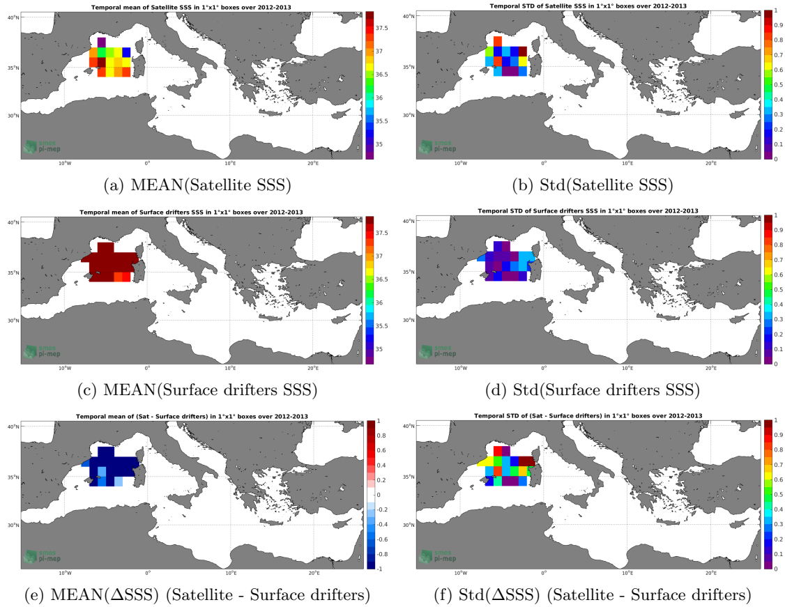
Figure 5: Temporal mean (left) and Std (right) of SSS from Aquarius-L3-OR-V5-7DAY-RUNNING-RAIN-MASK-1DEG (top), Surface drifters (middle), and of \Delta SSS (Satellite - Surface drifters). Only match-up pairs are used to generate these maps.
