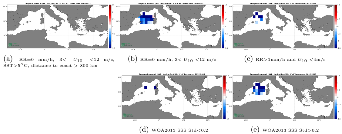
Figure 11: Temporal mean gridded over spatial boxes of size 1^\circ \times 1^\circ of \Delta SSS (Aquarius-L3-OR-V5-7DAY-RUNNING-RAIN-MASK-1DEG - Surface drifters) for 5 different subdatasets corresponding to:RR=0 mm/h, 3 < U_{10} < 12 m/s, SST >5^\circ\text{C} , distance to coast > 800 km (a), RR=0 mm/h, 3 < U_{10} < 12 m/s (b), RR >1 mm/h and U_{10} < 4 m/s (c), WOA2013 SSS Std <0.2 (d), WOA2013 SSS Std >0.2 (e).
