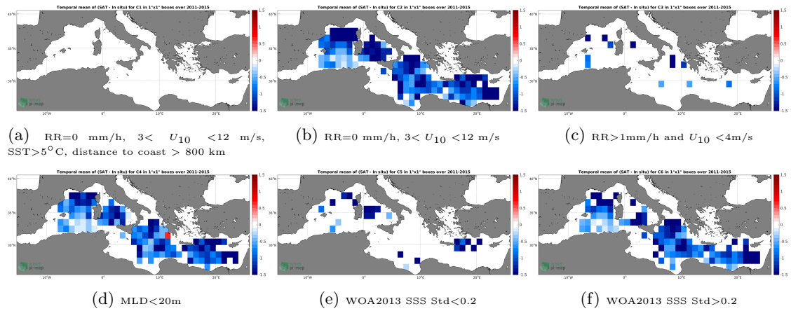
Figure 12: Temporal mean gridded over spatial boxes of size 1°x1° of \Delta SSS (Aquarius-L3-OR-V5-7DAY-RUNNING-RAIN-MASK-1DEG - Argo) for 6 different subdatasets corresponding to:RR=0 mm/h, 3 < U_{10} < 12 m/s, SST>5°C, distance to coast > 800 km (a), RR=0 mm/h, 3 < U_{10} < 12 m/s (b), RR>1mm/h and U_{10} < 4m/s (c),MLD<20m (d),WOA2013 SSS Std<0.2 (e),WOA2013 SSS Std>0.2 (f).
