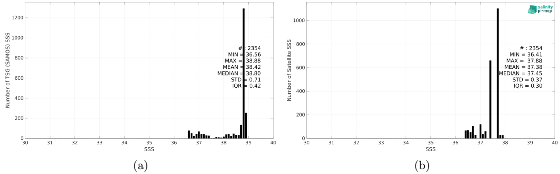
Figure 2: Histograms of SSS from TSG (SAMOS) (a) and Aquarius SSS L3 OR v5 - Monthly (NASA-GSFC) (b) considering all match-up pairs per bins of 0.1 over the Mediterranean Sea Pi-MEP region and for the full satellite product period.
