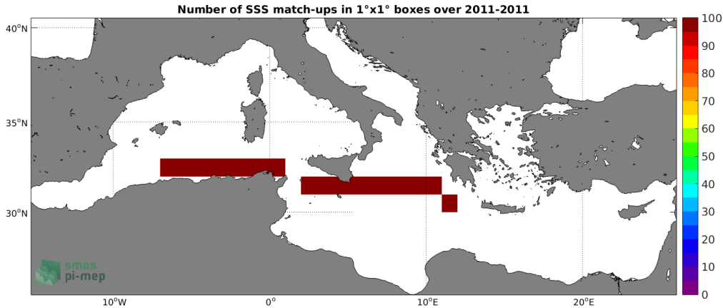
Figure 4: Number of SSS match-ups between TSG (SAMOS) SSS and the Aquarius SSS L3 OR v5 - Monthly (NASA-GSFC) SSS product for the Mediterranean Sea Pi-MEP region over 1^\circ \times 1^\circ boxes and for the full satellite product period.
