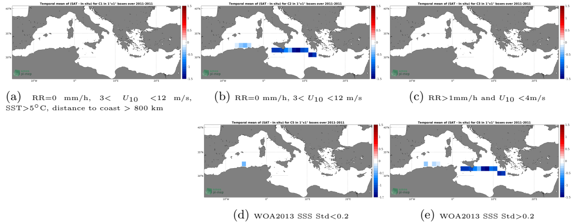
Figure 12: Temporal mean gridded over spatial boxes of size 1^{\circ}\times 1^{\circ} of \Delta\text{SSS} (Aquarius SSS L3 OR v5 - Monthly (NASA-GSFC) - TSG (SAMOS)) for 5 different subdatasets corresponding to:RR=0 mm/h, 3 < U_{10} < 12 m/s, SST >5^{\circ}\text{C} , distance to coast > 800 km (a), RR=0 mm/h, 3 < U_{10} < 12 m/s (b), RR >1 mm/h and U_{10} < 4 m/s (c), WOA2013 SSS Std <0.2 (d), WOA2013 SSS Std >0.2 (e).
