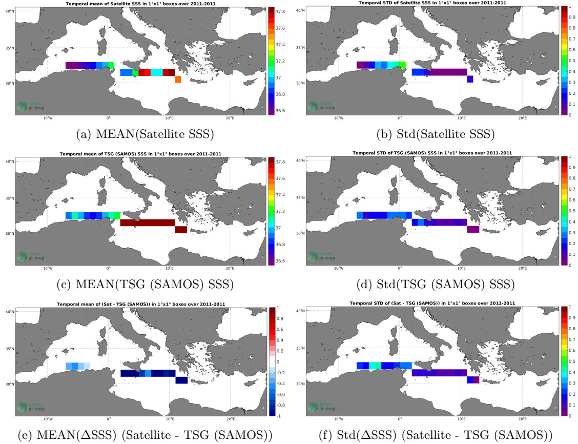
Figure 6: Temporal mean (left) and Std (right) of SSS from Aquarius SSS L3 OR v5 - Monthly (NASA-GSFC) (top), TSG (SAMOS) (middle), and of \Delta\text{SSS} (Satellite - TSG (SAMOS)). Only match-up pairs are used to generate these maps.
