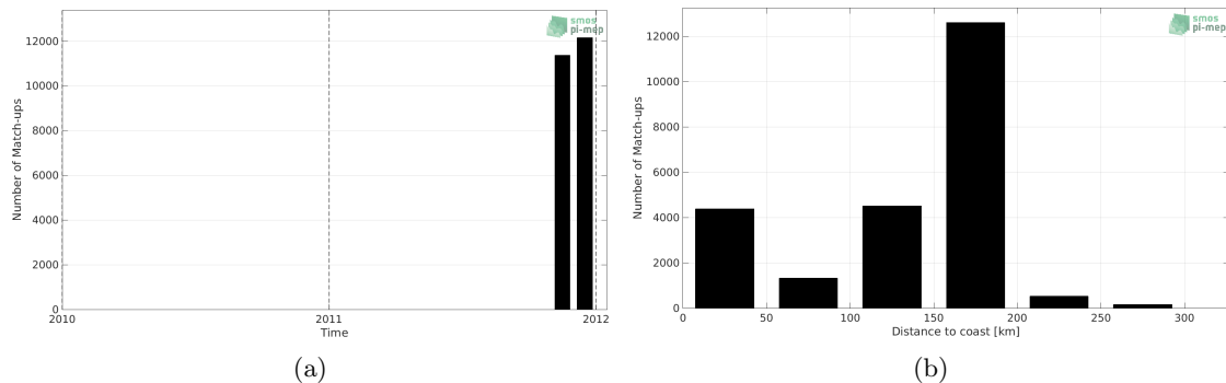
Figure 1: Number of match-ups between TSG (SAMOS) and Aquarius SSS L3 OR v5 - Monthly (NASA-GSFC) SSS as a function of time (a) and as function of the distance to coast (b) over the Mediterranean Sea Pi-MEP region and for the full satellite product period.
