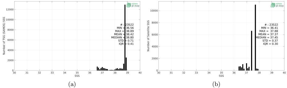
Figure 2: Histograms of SSS from TSG (SAMOS) (a) and Aquarius SSS L3 OR v5 - Monthly (NASA-GSFC) (b) considering all match-up pairs per bins of 0.1 over the Mediterranean Sea Pi-MEP region and for the full satellite product period.
