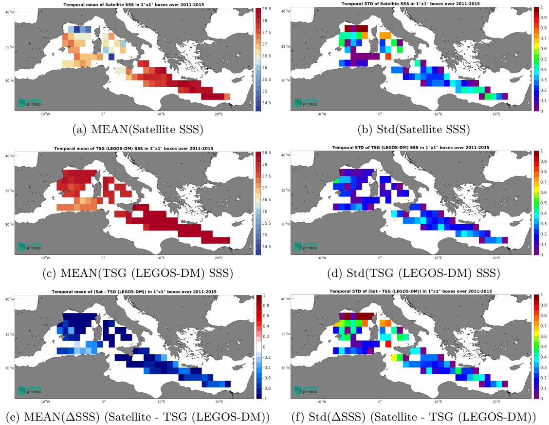
Figure 7: Temporal mean (left) and Std (right) of SSS from Aquarius SSS L3 OR v5 - Monthly (NASA-GSFC) (top), TSG (LEGOS-DM) ( in situ ) (middle), and of \Delta\text{SSS} (Satellite - TSG (LEGOS-DM)). Only match-up pairs are used to generate these maps.
