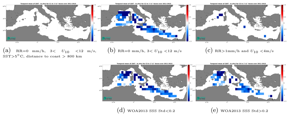
Figure 14: Temporal mean gridded over spatial boxes of size 1^\circ \times 1^\circ of \Delta SSS (Aquarius SSS L3 OR v5 - Monthly (NASA-GSFC) - TSG (LEGOS-DM)) for 5 different subdatasets corresponding to:RR=0 mm/h, 3 < U_{10} < 12 m/s, SST>5°C, distance to coast > 800 km (a), RR=0 mm/h, 3 < U_{10} < 12 m/s (b), RR>1mm/h and U_{10} < 4 m/s (c), WOA2013 SSS Std<0.2 (d), WOA2013 SSS Std>0.2 (e).
