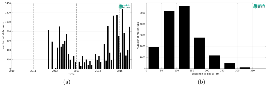
Figure 2: Number of match-ups between TSG (LEGOS-DM) and Aquarius SSS L3 OR v5 - Monthly (NASA-GSFC) SSS as a function of time (a) and as function of the distance to coast (b) over the Mediterranean Sea Pi-MEP region and for the full satellite product period.
