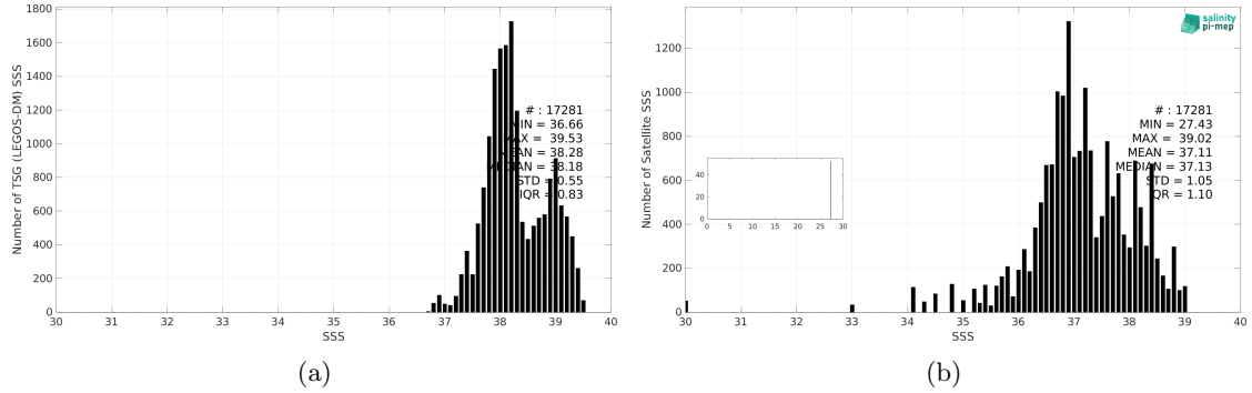
Figure 3: Histograms of SSS from TSG (LEGOS-DM) (a) and Aquarius SSS L3 OR v5 - Monthly (NASA-GSFC) (b) considering all match-up pairs per bins of 0.1 over the Mediterranean Sea Pi-MEP region and for the full satellite product period.
