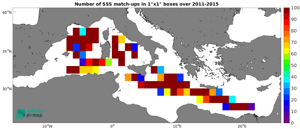
Figure 5: Number of SSS match-ups between TSG (LEGOS-DM) SSS and the Aquarius SSS L3 OR v5 - Monthly (NASA-GSFC) SSS product for the Mediterranean Sea Pi-MEP region over 1^\circ \times 1^\circ boxes and for the full satellite product period.
