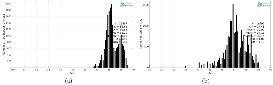
Figure 2: Histograms of SSS from TSG (LEGOS-DM) (a) and Aquarius SSS L3 OR v5 - Monthly (NASA-GSFC) (b) considering all match-up pairs per bins of 0.1 over the Mediterranean Sea Pi-MEP region and for the full satellite product period.
