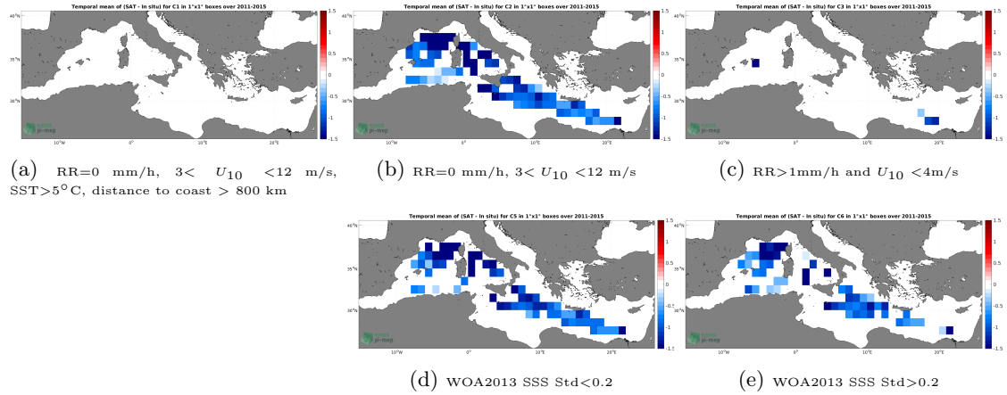
Figure 12: Temporal mean gridded over spatial boxes of size 1^{\circ}\times 1^{\circ} of \Delta\text{SSS} (Aquarius SSS L3 OR v5 - Monthly (NASA-GSFC) - TSG (LEGOS-DM)) for 5 different subdatasets corresponding to:RR=0 mm/h, 3 < U_{10} < 12 m/s, SST > 5^{\circ}\text{C} , distance to coast > 800 km (a), RR=0 mm/h, 3 < U_{10} < 12 m/s (b), RR > 1 mm/h and U_{10} < 4 m/s (c), WOA2013 SSS Std < 0.2 (d), WOA2013 SSS Std > 0.2 (e).
