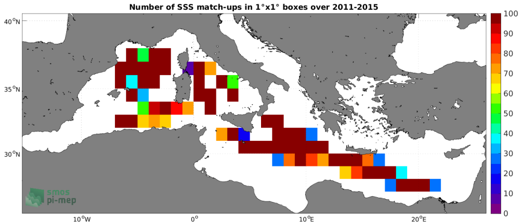
Figure 4: Number of SSS match-ups between TSG (LEGOS-DM) SSS and the Aquarius SSS L3 OR v5 - Monthly (NASA-GSFC) SSS product for the Mediterranean Sea Pi-MEP region over 1^\circ \times 1^\circ boxes and for the full satellite product period.
