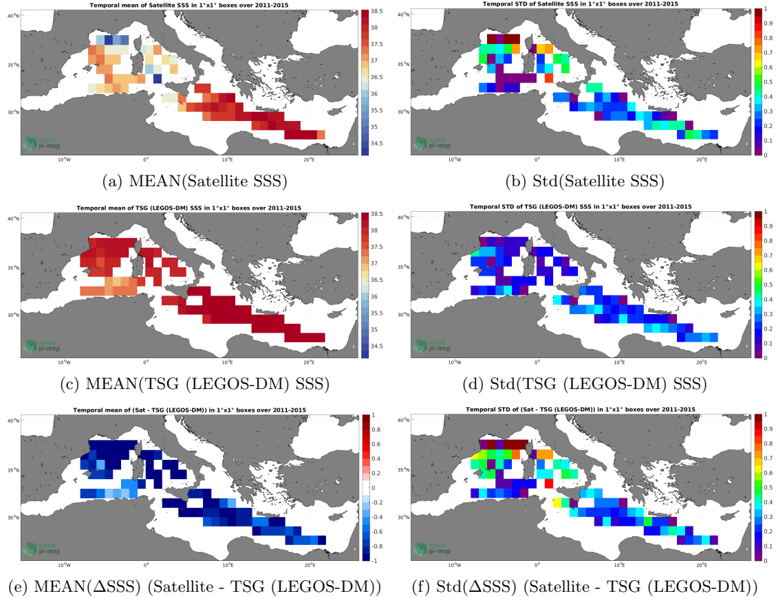
Figure 6: Temporal mean (left) and Std (right) of SSS from Aquarius SSS L3 OR v5 - Monthly (NASA-GSFC) (top), TSG (LEGOS-DM) ( in situ ) (middle), and of \Delta\text{SSS} (Satellite - TSG (LEGOS-DM)). Only match-up pairs are used to generate these maps.
