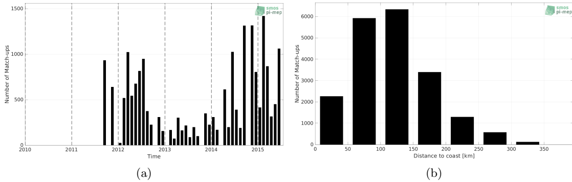
Figure 1: Number of match-ups between TSG (LEGOS-DM) and Aquarius SSS L3 OR v5 - Monthly (NASA-GSFC) SSS as a function of time (a) and as function of the distance to coast (b) over the Mediterranean Sea Pi-MEP region and for the full satellite product period.
