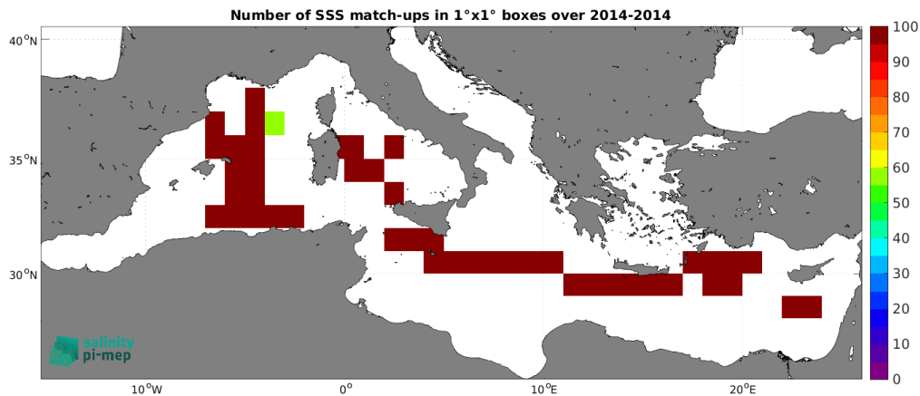
Figure 5: Number of SSS match-ups between TSG (GOSUD-Sailing-ship) SSS and the Aquarius SSS L3 OR v5 - Monthly (NASA-GSFC) SSS product for the Mediterranean Sea Pi-MEP region over 1^\circ \times 1^\circ boxes and for the full satellite product period.
