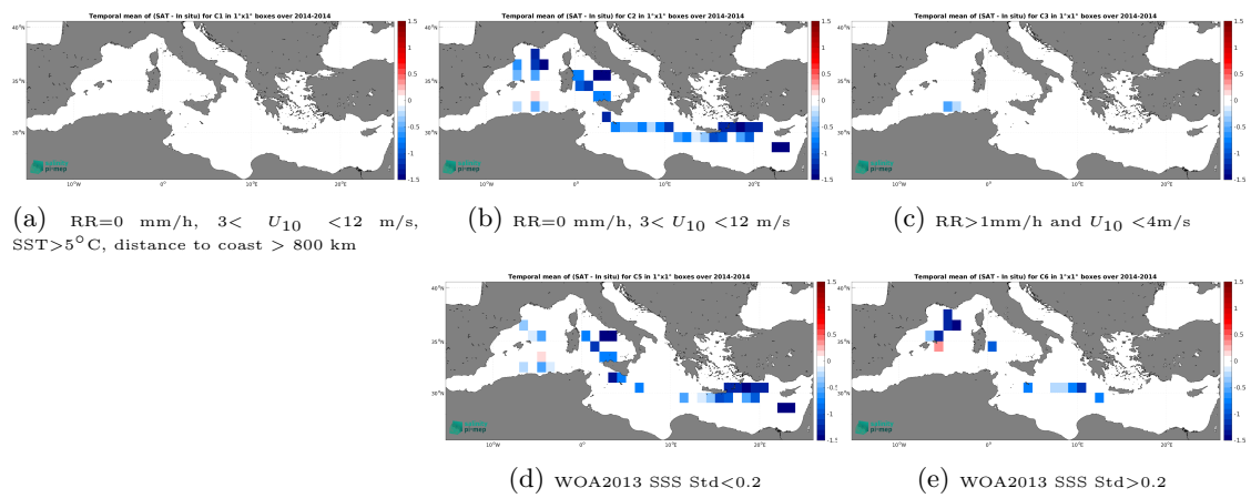
Figure 14: Temporal mean gridded over spatial boxes of size 1^\circ \times 1^\circ of \Delta SSS (Aquarius SSS L3 OR v5 - Monthly (NASA-GSFC) - TSG (GOSUD-Sailing-ship)) for 5 different subdatasets corresponding to:RR=0 mm/h, 3 < U_{10} < 12 m/s, SST >5^\circ\text{C} , distance to coast > 800 km (a), RR=0 mm/h, 3 < U_{10} < 12 m/s (b), RR >1 mm/h and U_{10} < 4 m/s (c), WOA2013 SSS Std <0.2 (d), WOA2013 SSS Std >0.2 (e).
