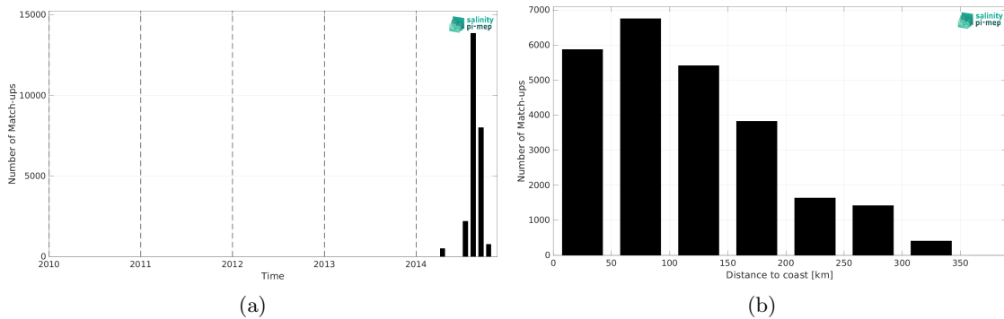
Figure 2: Number of match-ups between TSG (GOSUD-Sailing-ship) and Aquarius SSS L3 OR v5 - Monthly (NASA-GSFC) SSS as a function of time (a) and as function of the distance to coast (b) over the Mediterranean Sea Pi-MEP region and for the full satellite product period.
