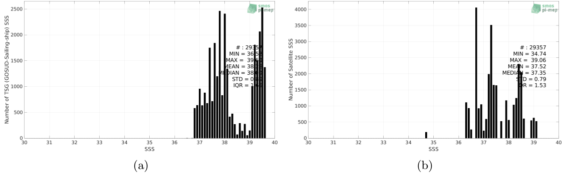
Figure 2: Histograms of SSS from TSG (GOSUD-Sailing-ship) (a) and Aquarius SSS L3 OR v5 - Monthly (NASA-GSFC) (b) considering all match-up pairs per bins of 0.1 over the Mediterranean Sea Pi-MEP region and for the full satellite product period.
