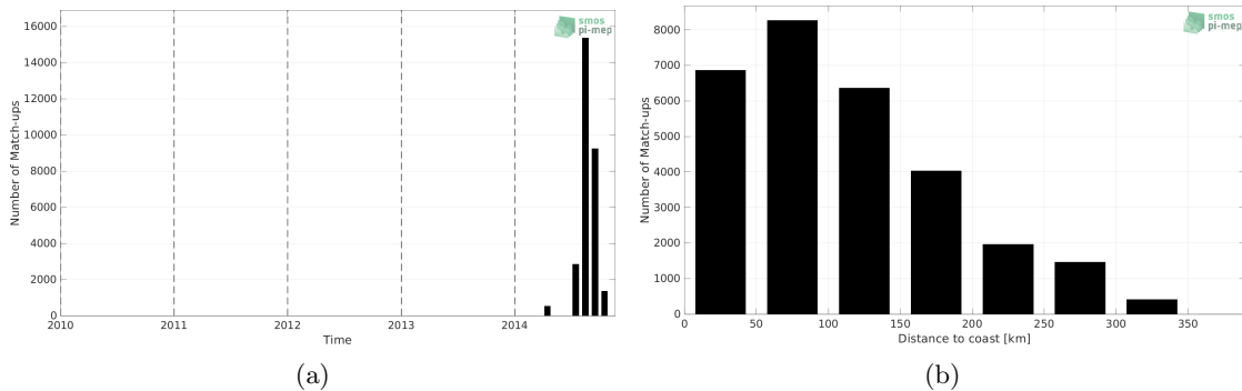
Figure 1: Number of match-ups between TSG (GOSUD-Sailing-ship) and Aquarius SSS L3 OR v5 - Monthly (NASA-GSFC) SSS as a function of time (a) and as function of the distance to coast (b) over the Mediterranean Sea Pi-MEP region and for the full satellite product period.
