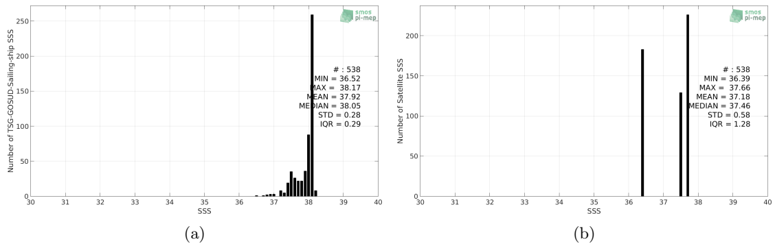
Figure 2: Histograms of SSS from TSG-GOSUD-Sailing-ship (a) and Aquarius-L3-OR-V5-MONTHLY-1DEG (b) considering all match-up pairs per bins of 0.1 over the Mediterranean Sea Pi-MEP region and for the full satellite product period.
