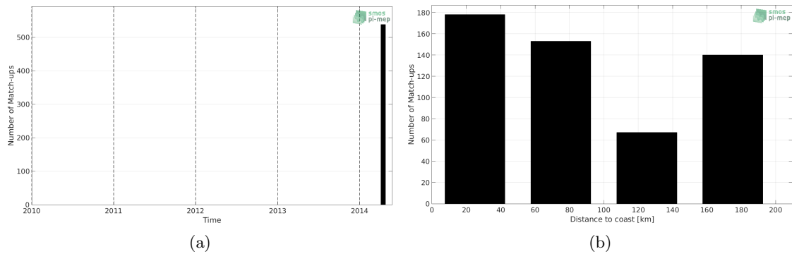
Figure 1: Number of match-ups between TSG-GOSUD-Sailing-ship and Aquarius-L3-OR-V5-MONTHLY-1DEG SSS as a function of time (a) and as function of the distance to coast (b) over the Mediterranean Sea Pi-MEP region and for the full satellite product period.
