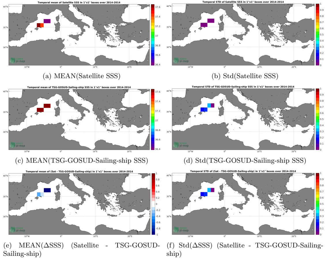
Figure 6: Temporal mean (left) and Std (right) of SSS from Aquarius-L3-OR-V5-MONTHLY-1DEG (top), TSG-GOSUD-Sailing-ship (middle), and of \Delta SSS (Satellite - TSG-GOSUD-Sailing-ship). Only match-up pairs are used to generate these maps.
