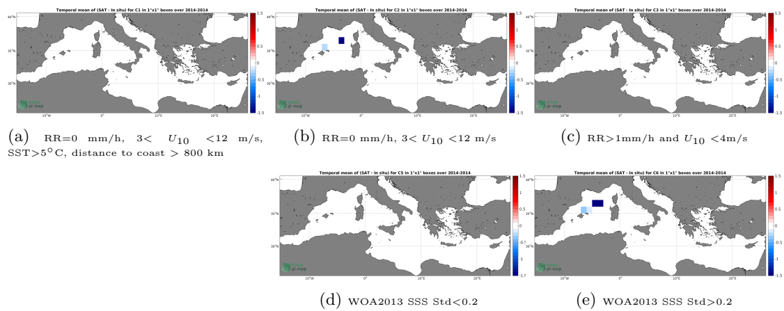
Figure 12: Temporal mean gridded over spatial boxes of size 1^\circ \times 1^\circ of \Delta SSS (Aquarius-L3-OR-V5-MONTHLY-1DEG - TSG-GOSUD-Sailing-ship) for 5 different subdatasets corresponding to:RR=0 mm/h, 3 < U_{10} < 12 m/s, SST>5°C, distance to coast > 800 km (a), RR=0 mm/h, 3 < U_{10} < 12 m/s (b), RR>1mm/h and U_{10} < 4 m/s (c), WOA2013 SSS Std<0.2 (d), WOA2013 SSS Std>0.2 (e).
