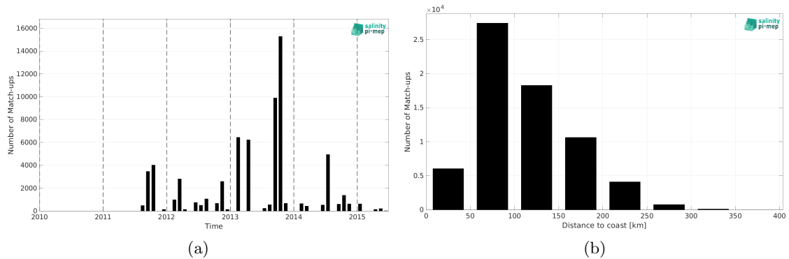
Figure 2: Number of match-ups between TSG (GOSUD-Research-vessel) and Aquarius SSS L3 OR v5 - Monthly (NASA-GSFC) SSS as a function of time (a) and as function of the distance to coast (b) over the Mediterranean Sea Pi-MEP region and for the full satellite product period.
