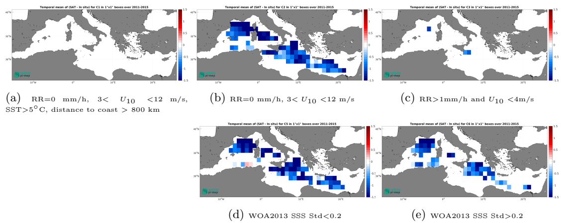
Figure 14: Temporal mean gridded over spatial boxes of size 1^\circ \times 1^\circ of \Delta SSS (Aquarius SSS L3 OR v5 - Monthly (NASA-GSFC) - TSG (GOSUD-Research-vessel)) for 5 different subdatasets corresponding to:RR=0 mm/h, 3 < U_{10} < 12 m/s, SST>5°C, distance to coast > 800 km (a), RR=0 mm/h, 3 < U_{10} < 12 m/s (b), RR>1mm/h and U_{10} < 4 m/s (c), WOA2013 SSS Std<0.2 (d), WOA2013 SSS Std>0.2 (e).
