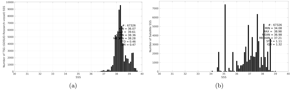
Figure 3: Histograms of SSS from TSG (GOSUD-Research-vessel) (a) and Aquarius SSS L3 OR v5 - Monthly (NASA-GSFC) (b) considering all match-up pairs per bins of 0.1 over the Mediterranean Sea Pi-MEP region and for the full satellite product period.
