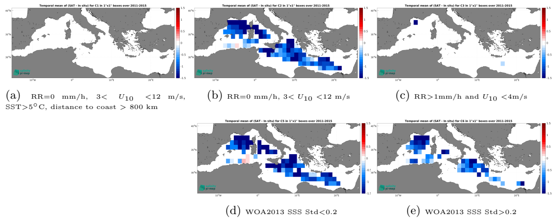
Figure 12: Temporal mean gridded over spatial boxes of size 1^{\circ}\times 1^{\circ} of \Delta SSS (Aquarius SSS L3 OR v5 - Monthly (NASA-GSFC) - TSG (GOSUD-Research-vessel)) for 5 different subdatasets corresponding to:RR=0 mm/h, 3 < U_{10} < 12 m/s, SST >5^{\circ}\text{C} , distance to coast > 800 km (a), RR=0 mm/h, 3 < U_{10} < 12 m/s (b), RR >1 mm/h and U_{10} < 4 m/s (c), WOA2013 SSS Std <0.2 (d), WOA2013 SSS Std >0.2 (e).
