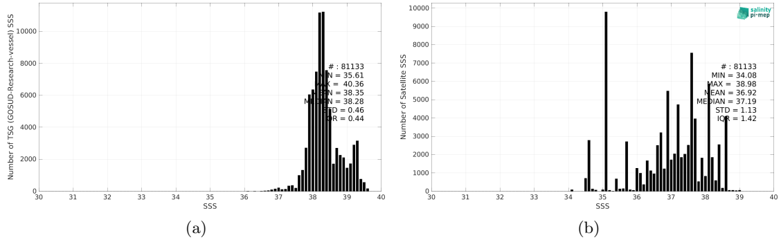
Figure 2: Histograms of SSS from TSG (GOSUD-Research-vessel) (a) and Aquarius SSS L3 OR v5 - Monthly (NASA-GSFC) (b) considering all match-up pairs per bins of 0.1 over the Mediterranean Sea Pi-MEP region and for the full satellite product period.
