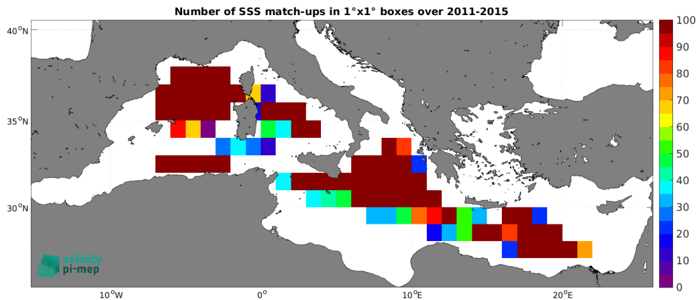
Figure 4: Number of SSS match-ups between TSG (GOSUD-Research-vessel) SSS and the Aquarius SSS L3 OR v5 - Monthly (NASA-GSFC) SSS product for the Mediterranean Sea Pi-MEP region over 1^\circ \times 1^\circ boxes and for the full satellite product period.
