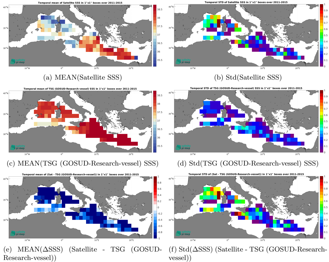
Figure 6: Temporal mean (left) and Std (right) of SSS from Aquarius SSS L3 OR v5 - Monthly (NASA-GSFC) (top), TSG (GOSUD-Research-vessel) (middle), and of \Delta\text{SSS} (Satellite - TSG (GOSUD-Research-vessel)). Only match-up pairs are used to generate these maps.
