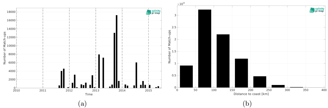
Figure 1: Number of match-ups between TSG (GOSUD-Research-vessel) and Aquarius SSS L3 OR v5 - Monthly (NASA-GSFC) SSS as a function of time (a) and as function of the distance to coast (b) over the Mediterranean Sea Pi-MEP region and for the full satellite product period.
