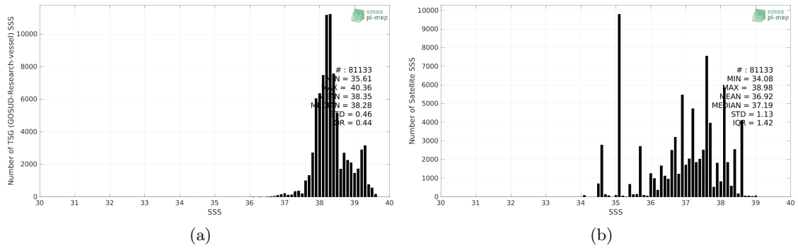
Figure 2: Histograms of SSS from TSG (GOSUD-Research-vessel) (a) and Aquarius SSS L3 OR v5 - Monthly (NASA-GSFC) (b) considering all match-up pairs per bins of 0.1 over the Mediterranean Sea Pi-MEP region and for the full satellite product period.
