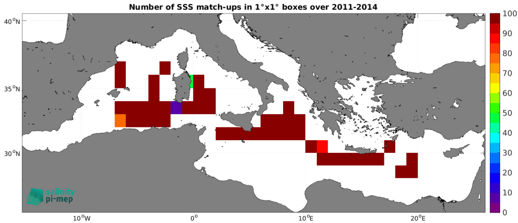
Figure 5: Number of SSS match-ups between TSG (CSIC-UTM) SSS and the Aquarius SSS L3 OR v5 - Monthly (NASA-GSFC) SSS product for the Mediterranean Sea Pi-MEP region over 1^\circ \times 1^\circ boxes and for the full satellite product period.
