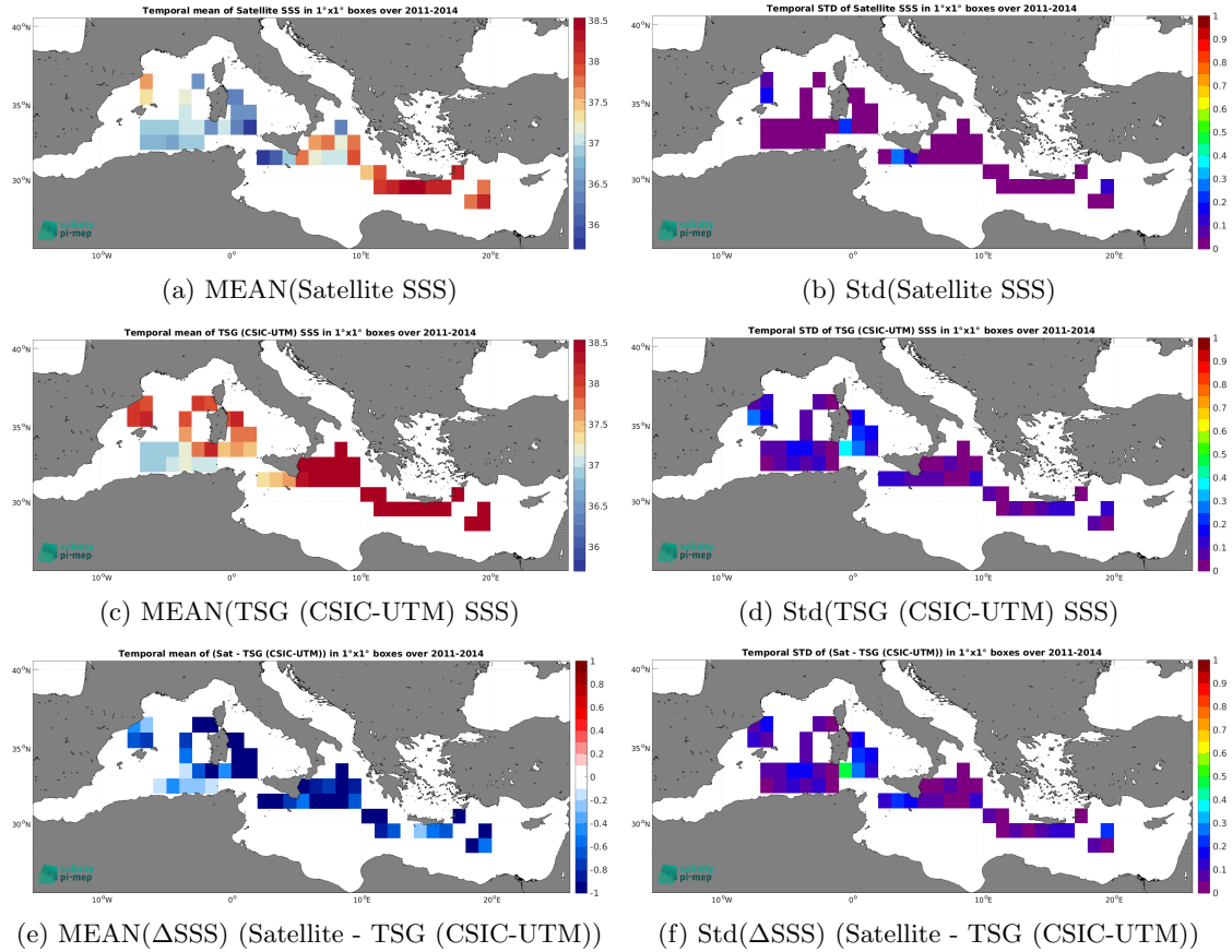
Figure 7: Temporal mean (left) and Std (right) of SSS from Aquarius SSS L3 OR v5 - Monthly (NASA-GSFC) (top), TSG (CSIC-UTM) ( in situ ) (middle), and of \Delta\text{SSS} (Satellite - TSG (CSIC-UTM)). Only match-up pairs are used to generate these maps.
