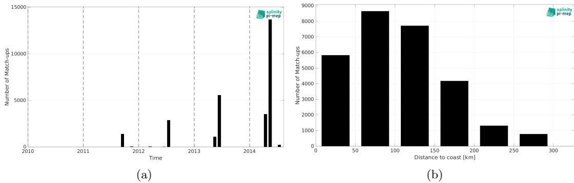
Figure 2: Number of match-ups between TSG (CSIC-UTM) and Aquarius SSS L3 OR v5 - Monthly (NASA-GSFC) SSS as a function of time (a) and as function of the distance to coast (b) over the Mediterranean Sea Pi-MEP region and for the full satellite product period.
