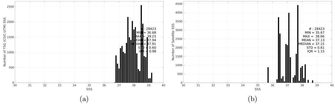
Figure 3: Histograms of SSS from TSG (CSIC-UTM) (a) and Aquarius SSS L3 OR v5 - Monthly (NASA-GSFC) (b) considering all match-up pairs per bins of 0.1 over the Mediterranean Sea Pi-MEP region and for the full satellite product period.
